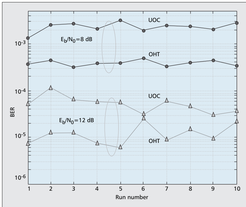
Figure 6. 802.16 BER vs. simulation run number for OHT and UOC V2V channels.
