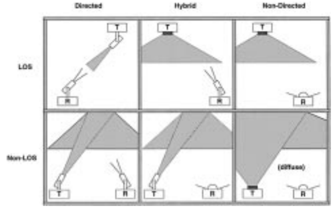
Fig. 2. Configurations for wireless infrared links. Nondirected, non-line-of-sight, or diffuse systems are considered here.
