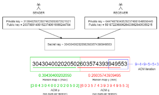
Figure 2: Illustration of initial value generation
