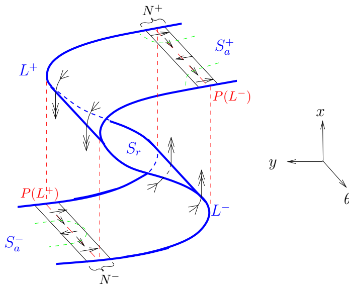
Figure 1. The critical manifold S and fold-curves L^\pm .
