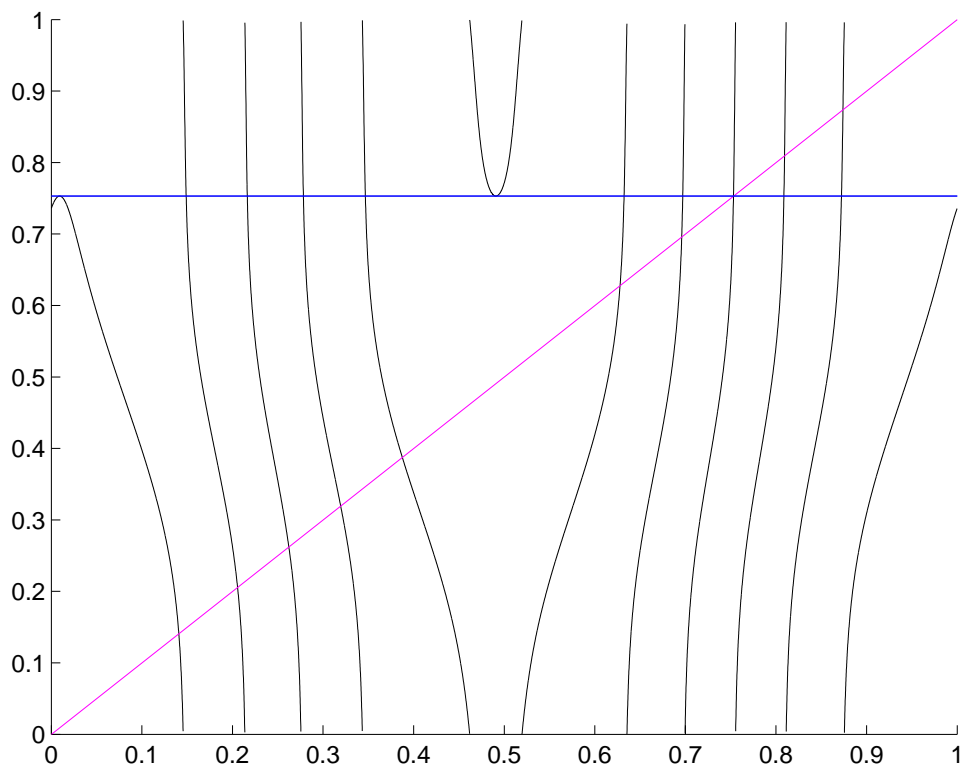
Figure 5. The graph of h
