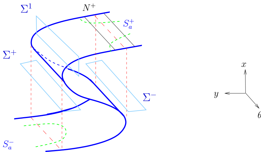
Figure 2. Poincaré section \Sigma^- of the map \Pi : \Sigma^- \rightarrow \Sigma^- and auxiliary sections \Sigma^+ and \Sigma^1
