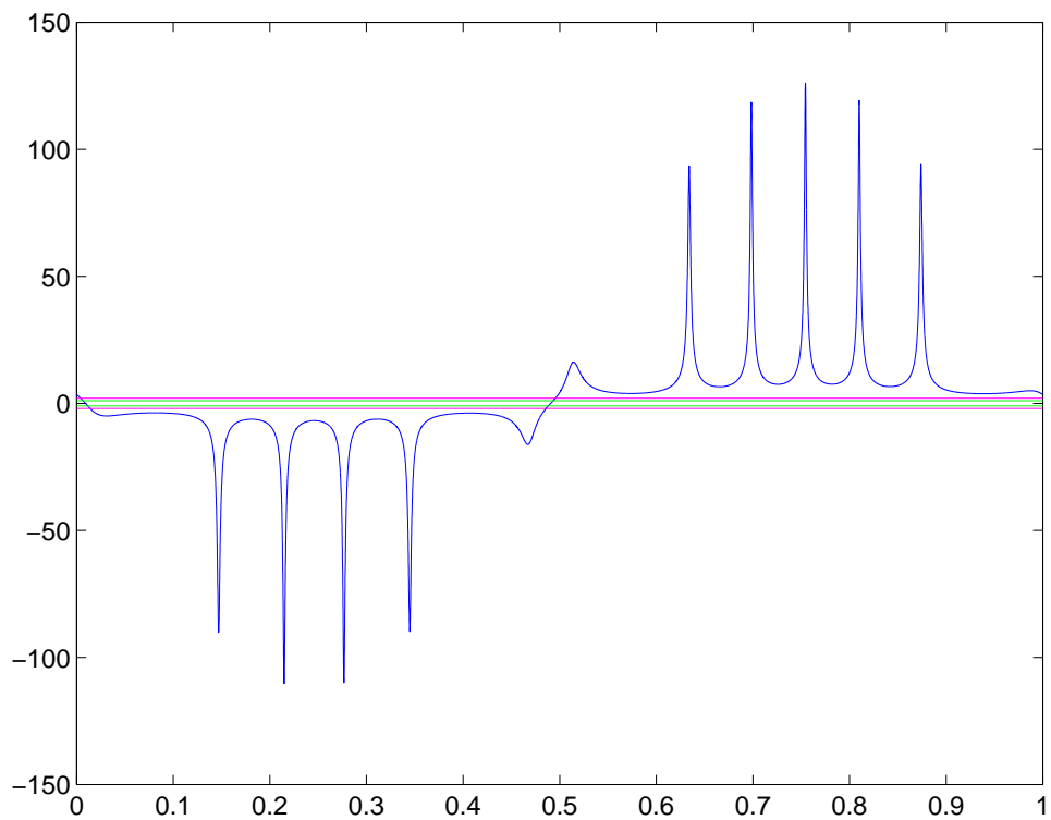
Figure 6. The graph of h'
