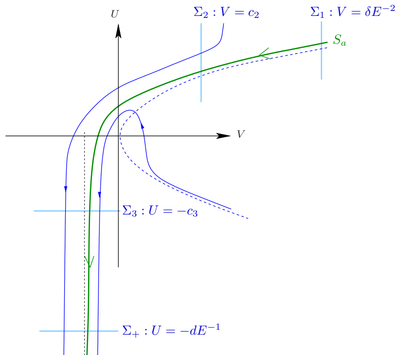
Figure 4. Sections in the rescaled system (15) in (U, V) phase space, which shows solutions of the Riccati equation (given by E = 0 in (15)). The special solution (green curve) of the Riccati equation represents the extension of the manifold S_a past the fold-curve
