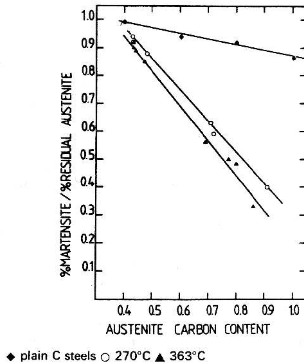
Figure 1.9: The austenite stability parameter as a function of carbon content, in wt% [49].
