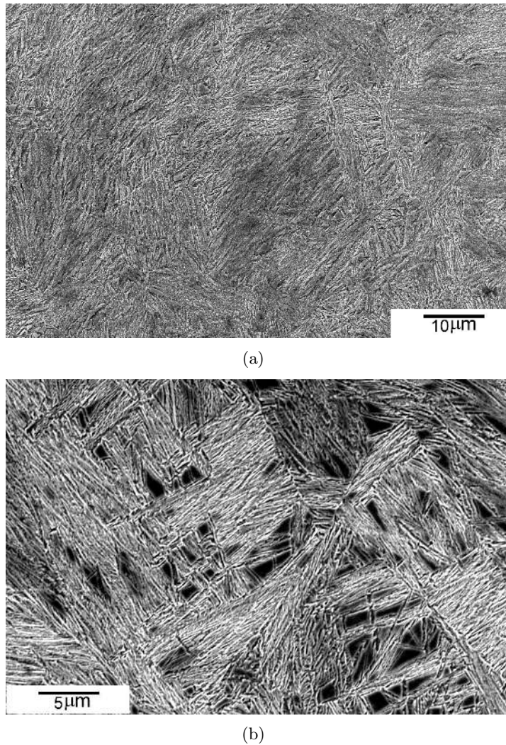
Figure A.6: SEM micrographs exhibit: (a) sample Sp9c, unstrained and tempered and (b) same sample, untempered. Samples underwent bainite transformation at 250°C for 15 h prior to DSC experiment. Tempering was carried out within the range 100°C to 600°C with the rate 10°C min -1 . Note the absence of the austenite in the tempered condition.
