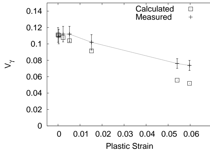
Figure B.3: Application of Sherif et al. model to experimental data from [184].
