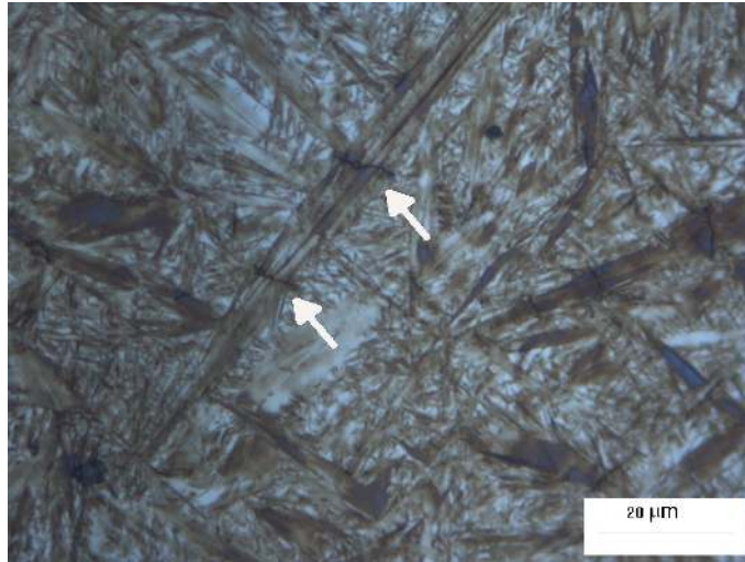
Figure 2.4: Sp10c microstructure featuring cracks generated in an athermal martensite plate (arrowed). The M_S temperature was calculated using MUCG73 and found to be 136^\circ\text{C} .
