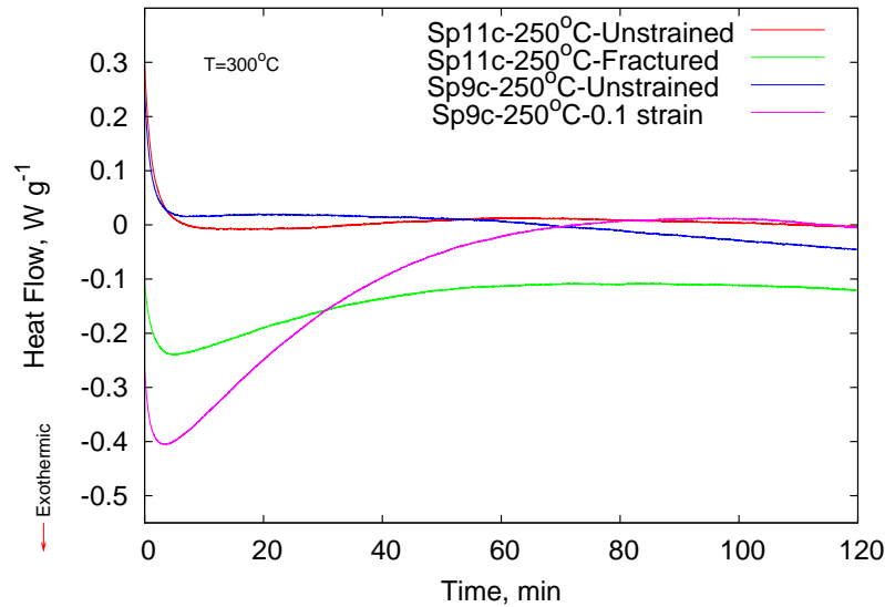
Figure A.11: Measured DSC curves in isothermal mode. See text for more details.
