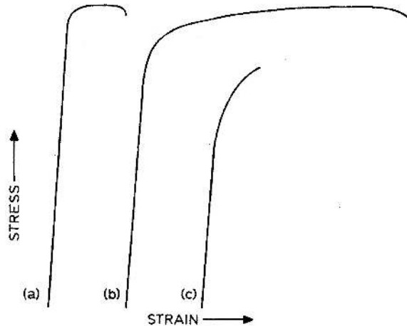
Figure 1.14: Stress-strain curves of steel with (a) low austenite volume fraction; (b) optimum volume fraction and (c) high volume fraction [92].
