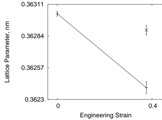
(a) Change in a_\gamma vs strain
