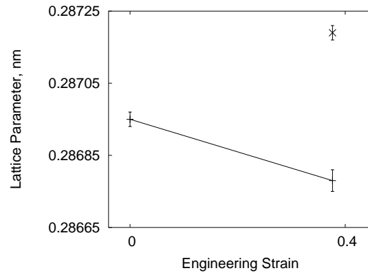
(b) Change in a_{\alpha_b} vs strain
