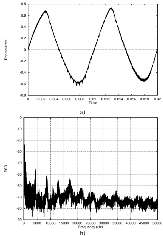
Figure 2. Fluorescent lamp interference: a) time waveform; b) spectrum.
