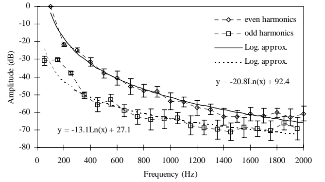
Figure 5. Average amplitude of each interference component.
