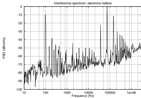
Figure 3. Spectrum of the interference produced by a fluorescent lamp geared by an electronic ballast.
