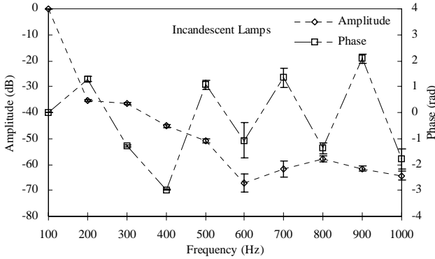
Figure 4. Average magnitude of the 100 Hz component and its harmonics.
