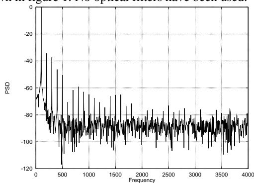
Figure 1. Typical interference spectrum of an incandescent lamp.
