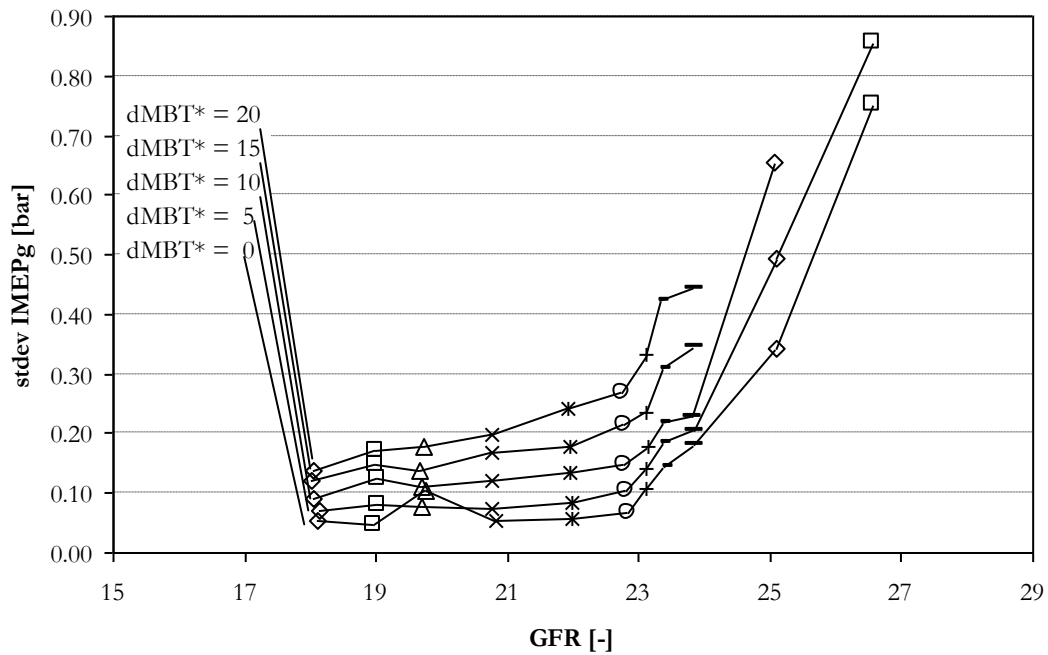
Figure 43 The influence of spark retard on stdev IMEPg over the same range of GFRs and engine conditions as shown in Figure 42.
