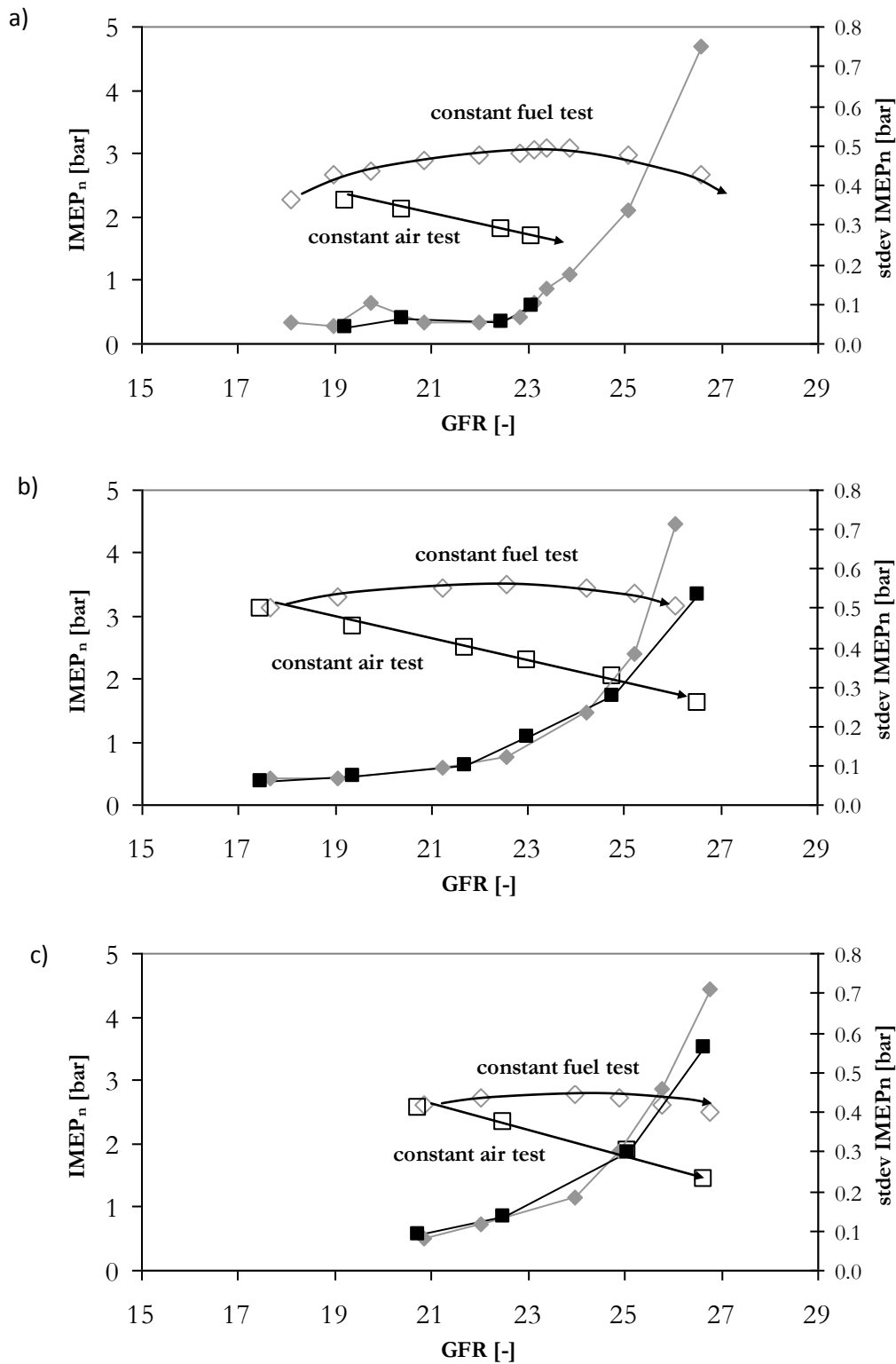
Figure 38 The change in IMEP n and stdev IMEP n with GFR for two different test methods, data as Figure 24. Constant fuel tests indicated with diamonds and constant air tests indicated with squares.
