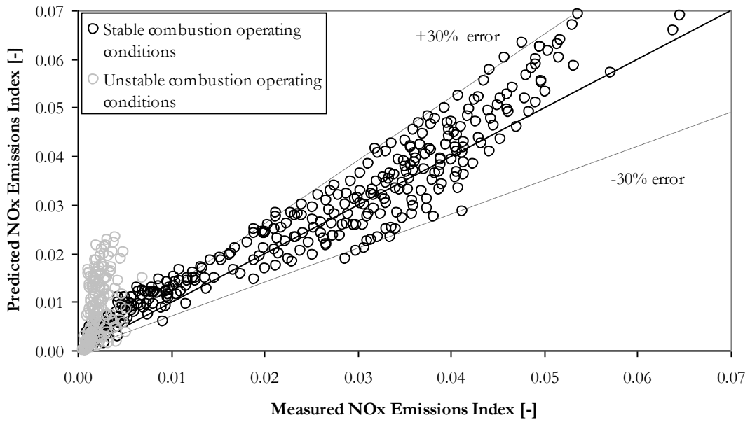
Figure 73 NOx Generic function performance for stable and unstable combustion operating conditions.
