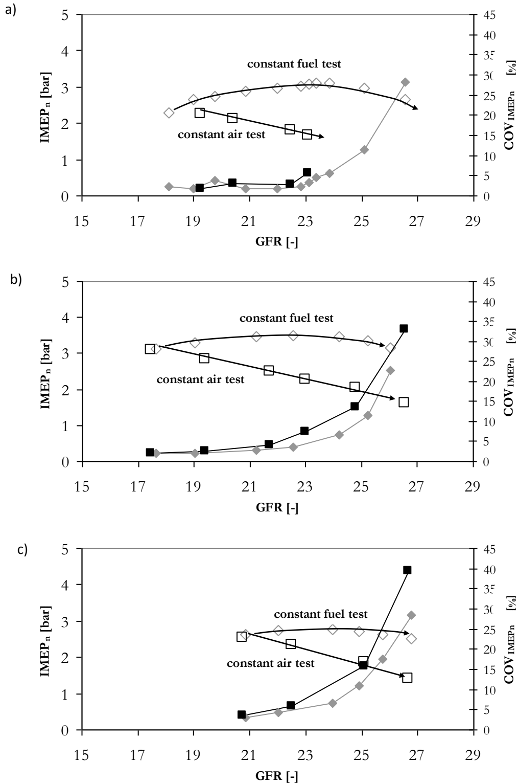
Figure 37 The change in IMEP n and COV IMEP n with GFR for two different test methods, constant fuel tests indicated with diamonds and constant air tests indicated with squares. Where a) is 1000rpm, b) 1500rpm and c) 2000rpm.
