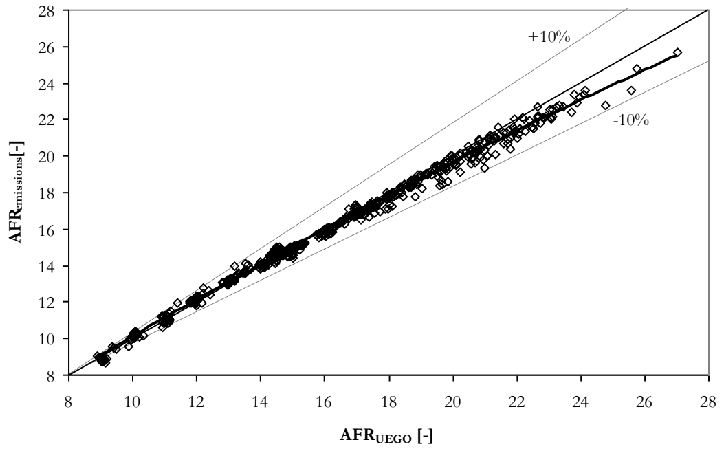
Figure 7 Comparison of AFR determined from the measured exhaust gas emissions and the UEGO sensor. Line of best fit through the data is shown, indicating a divergence from the y=x at lean operating conditions. Data includes engine speeds from idle to 4000rpm WOT and the full range of cam timings.
