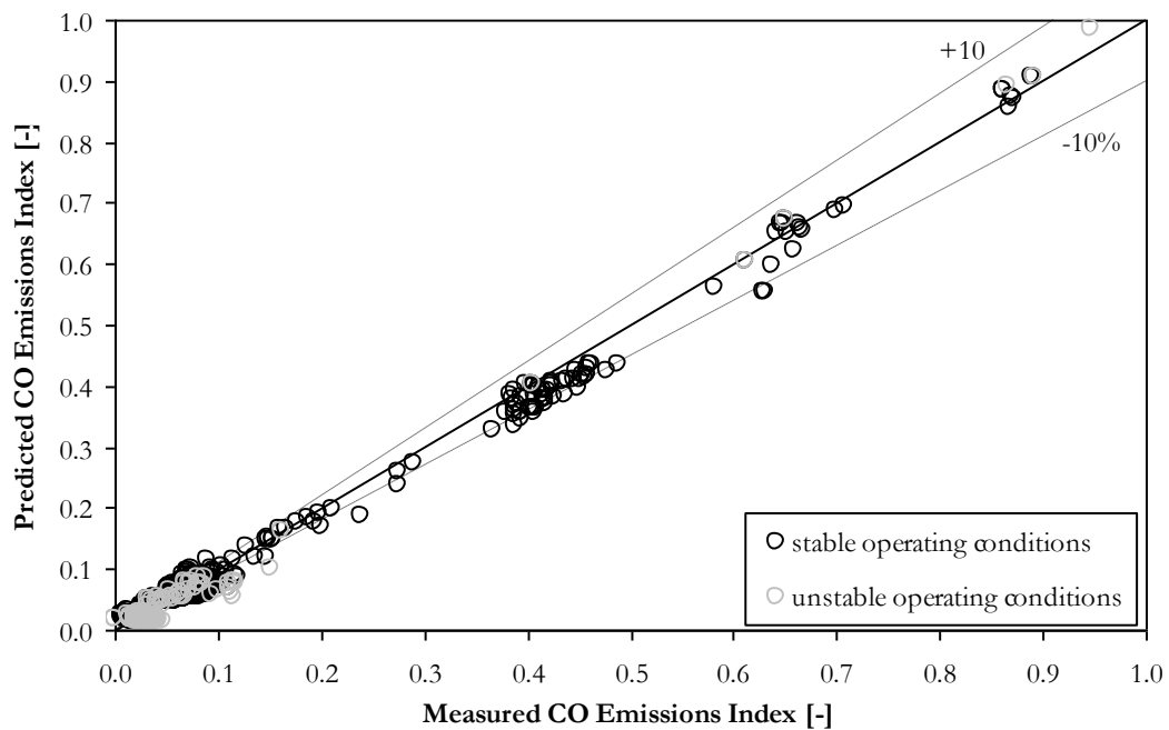
Figure 58 Performance of the carbon monoxide generic function for both unstable and stable operating points (where unstable is defined as COV_{IMEP} > 10 ).
