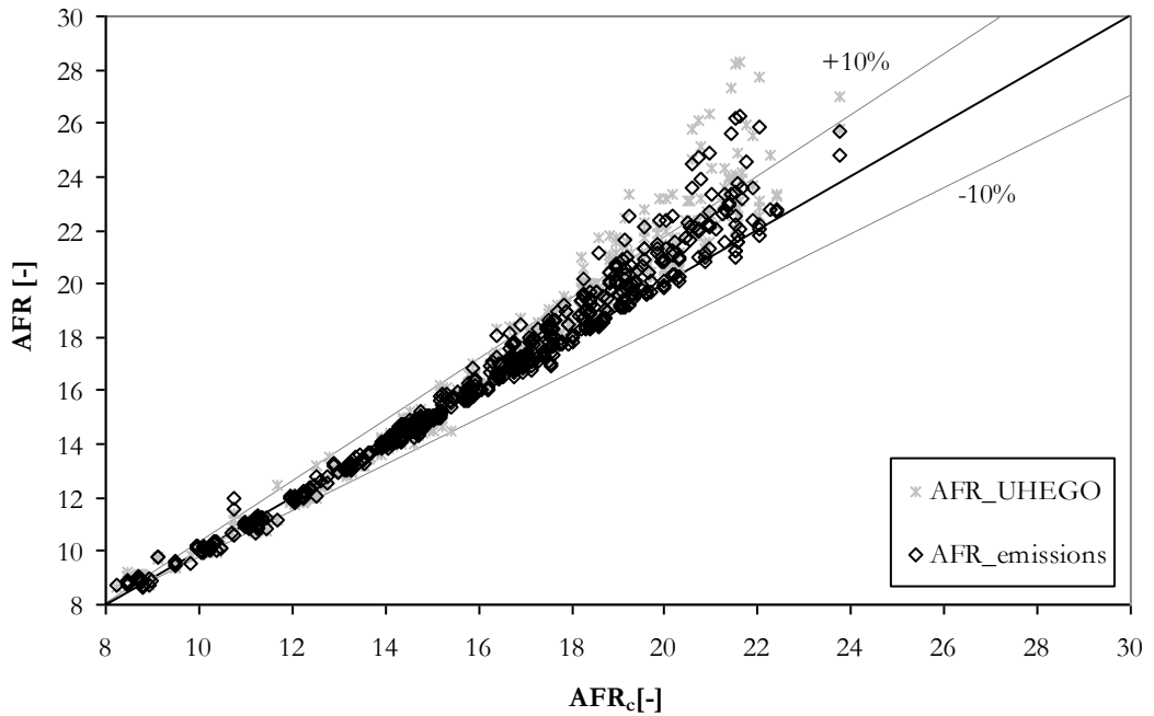
Figure 8 Relative inaccuracies of the AFR measured by the emissions and the UEGO sensor. AFR_c is calculated from equation 9, directly from the measured fuel pulse width.
