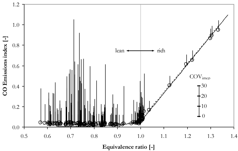
Figure 57 AJ27 carbon monoxide emissions index including operating point stability information ( COV_{IMEP} ). Height of each bar at each test point indicates the level of COV_{IMEP} , higher the bar greater the level of instability.
