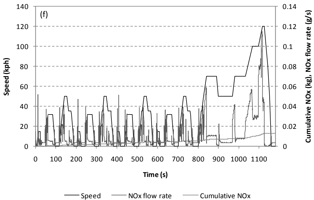
Figure 76 Influence of new emissions models over the NEDC. In all three cases the new model is shown before the original. (a) and (b) comparing CO emissions, (c) and (d) HC emissions, (e) and (f) NOx emissions
