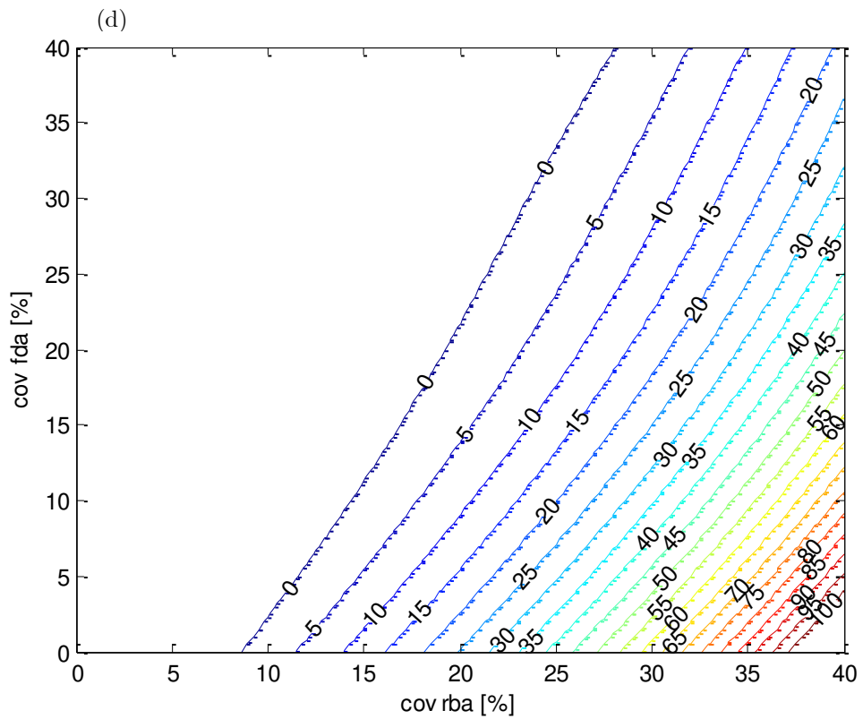
The effect of changes of COV_{\Delta\theta_{0-10\%}} and COV_{\Delta\theta_{10-90\%}} on COV_{IMEP_g} at five increasing \theta_d : (a) 30, (b) 50, (c) 70, (d) 90, (e) 115.
