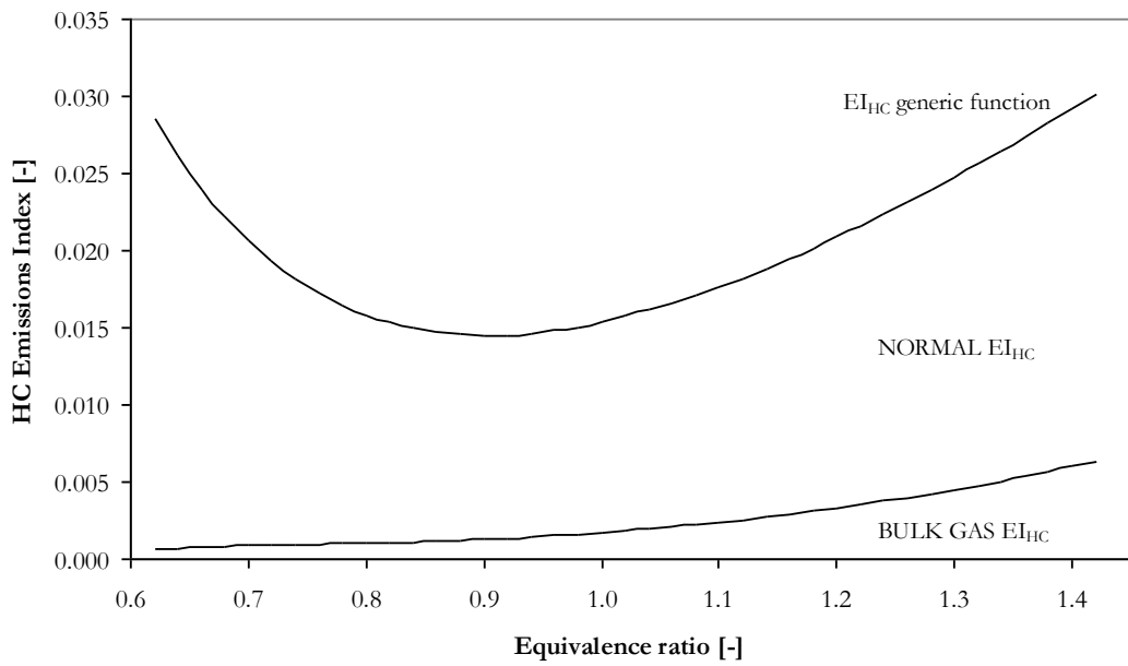
Figure 87 HC emissions index as a function of equivalence ratio
