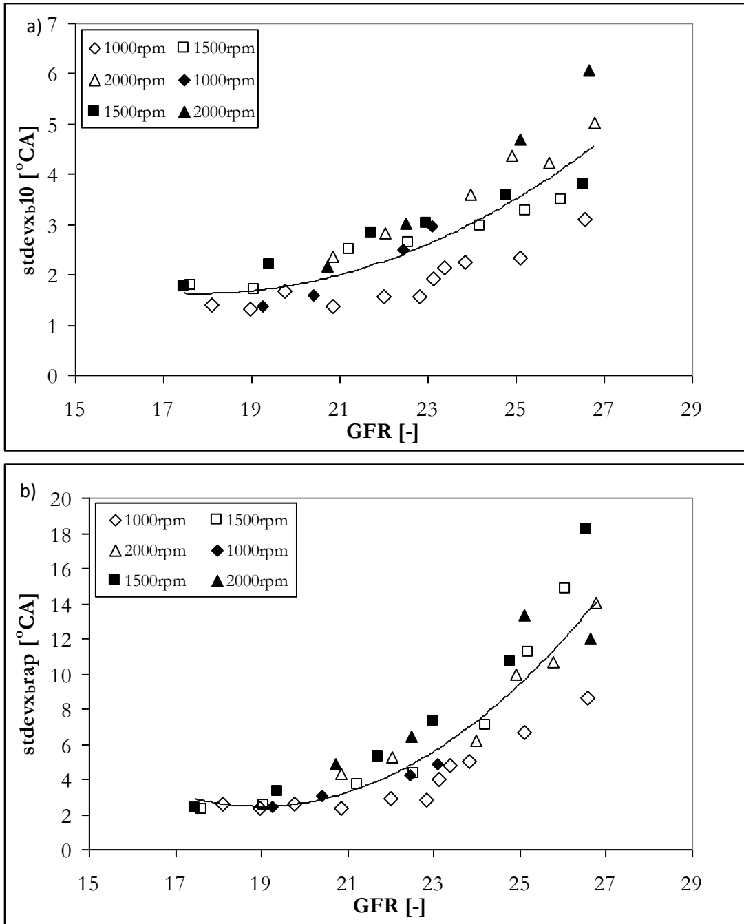
Figure 49 Change in (a) stdev\Delta\theta_{0-10\%} and (b) the stdev\Delta\theta_{10-90\%} with increasing GFR. Data shown as Figure 21.
