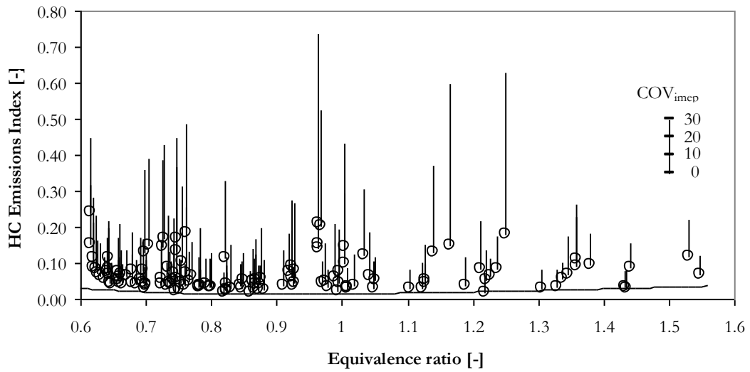
Figure 65 Effect of combustion instability on HC emissions index at MBT* operating conditions. The plotted line is generic function 2b. Height of each bar at each test point indicates the level of COV_{IMEP_n} , higher the bar greater the level of instability.
