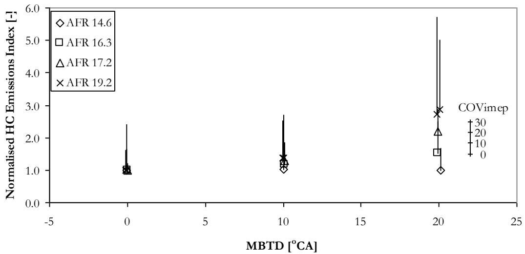
Figure 66 Effect of combustion instability reached by retarding the spark timing on HC emissions. Height of each bar at each test point indicates the level of COV_{IMEP_n} , higher the bar greater the level of instability.
