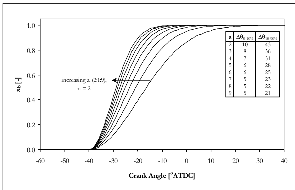
Figure 94 The effect of increasing a (efficiency factor) and n (form factor) on the shape of the burned mass fraction curve produced from the Wiebe function and the related changes in the x_{b,10} and x_{b,90} .
