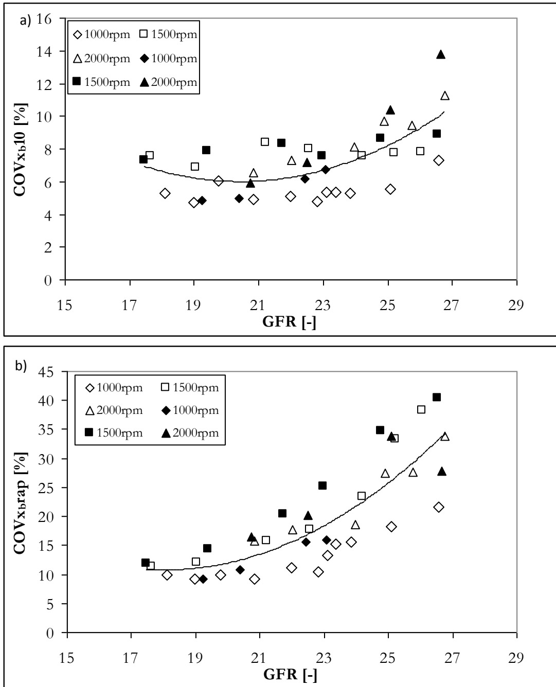
Figure 48 Change in (a) COV_{\Delta\theta_{-10\%}} and (b) the COV_{\Delta\theta_{10-90\%}} with increasing GFR. Open symbols constant fuel test points, filled symbols constant air test points. Values calculated as stated in Chapter 3.
