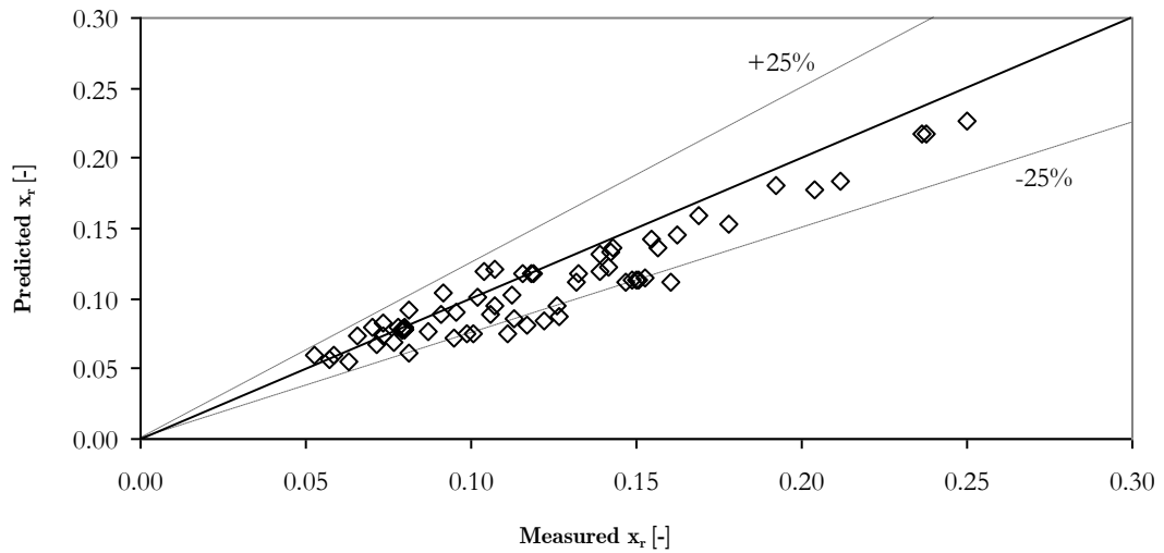
Figure 13 Comparison of the predicted x_r and the measured x_r . The predicted x_r is calculated from equation 27.
