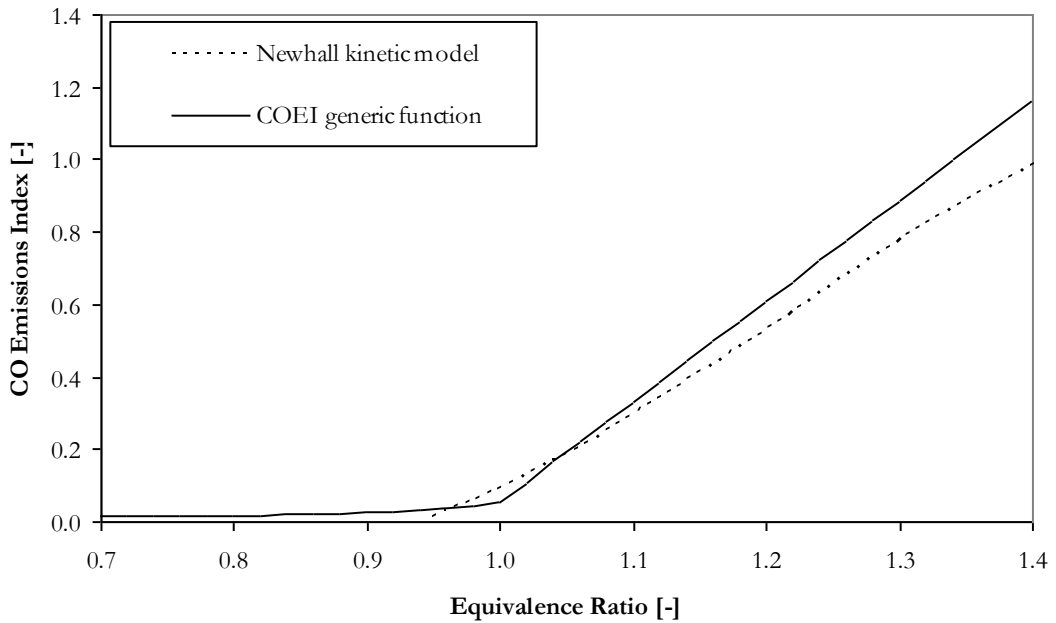
Figure 82 EI_{CO} , generic function and calculated at points throughout the cycle.
