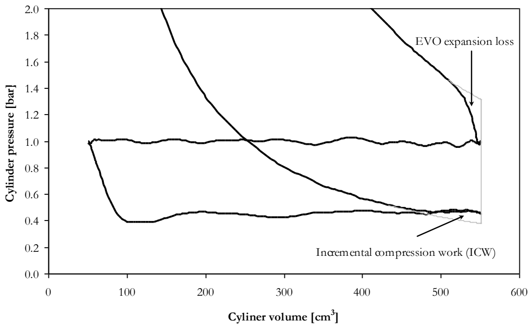
Figure 14 Example p vs. V diagram with extrapolated pressures allowing calculation of the EVO expansion loss and the incremental compression work. 1000rpm, IVC of 65°CA after BDC and EVO 40°CA BDC (equivalent to a -5°CA VO).
