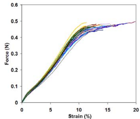
Figure 2: Load-strain curves for PET filaments
