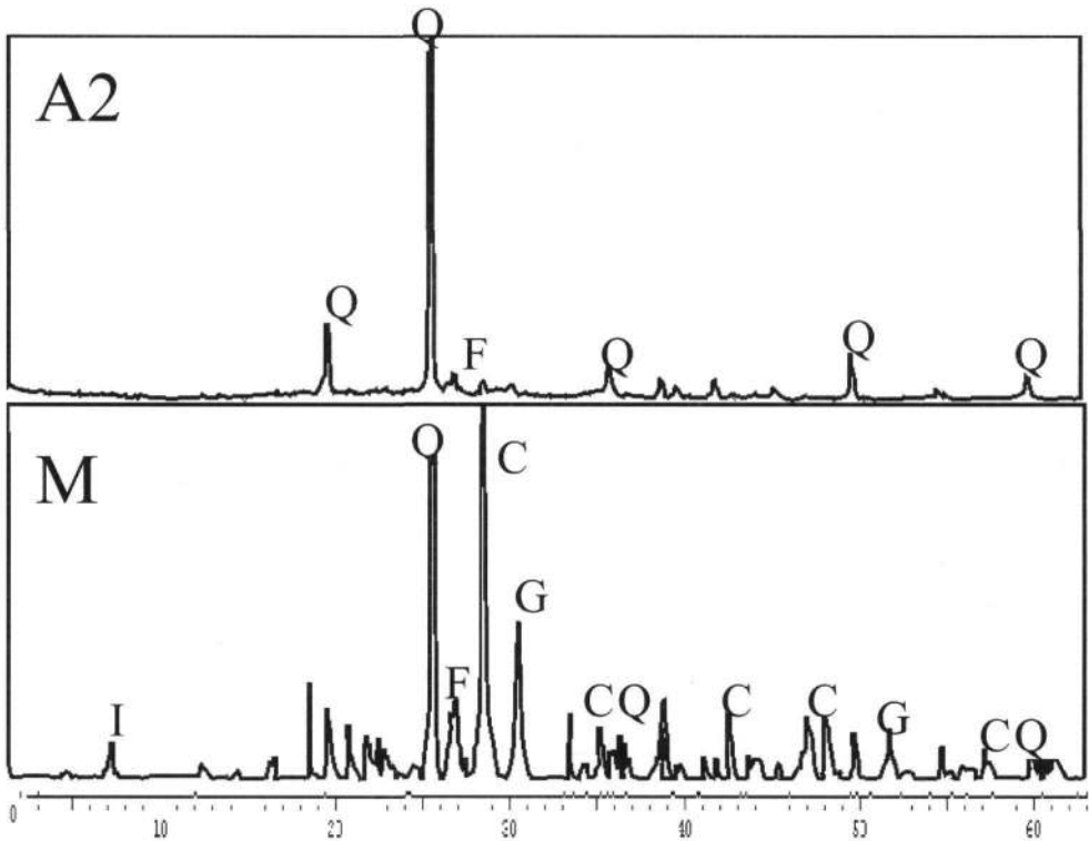
Figure 3 – XRD patterns of matt-painted (A2) and mycenaean pottery (M3) form Aiani, ancient upper Macedonia, Greece. (Q=quartz, F=feldspar, C=calcite, G=gehlenite, I=illite)
