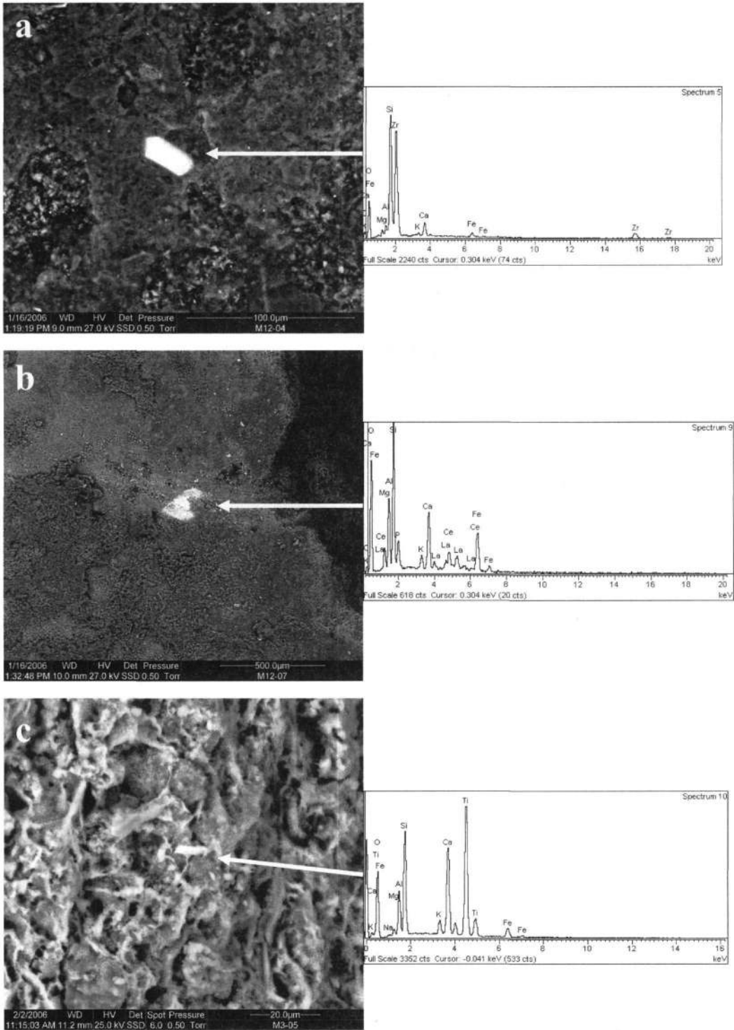
Figure 5 - ESEM images and EDX spectra of Mycenaean pottery: a) a zircon ( ZrSiO_4 ) crystal [M2 sample], b) a REE-rich (bright spots) inclusion [M2 sample], c) a titanite ( CaTiSiO_5 ) inclusion [M3 sample]
