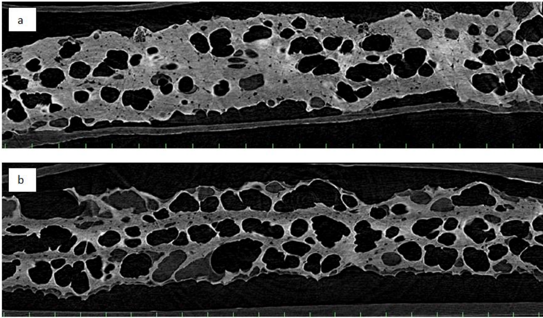
Fig. 6 - Micro-CT generated 2D image of (a) continuous fried kettle crisp, and (b) standard continuous fried crisp bottom, each notch on horizontal axis is 250 \mu m
