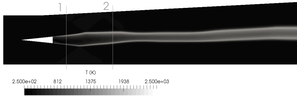
Figure 13: Temperature contour ( A_{\text{edm}} = 4, Pr_t = Sc_t = 0.9 ) with indication of the axial measurement locations considered in the present work.
