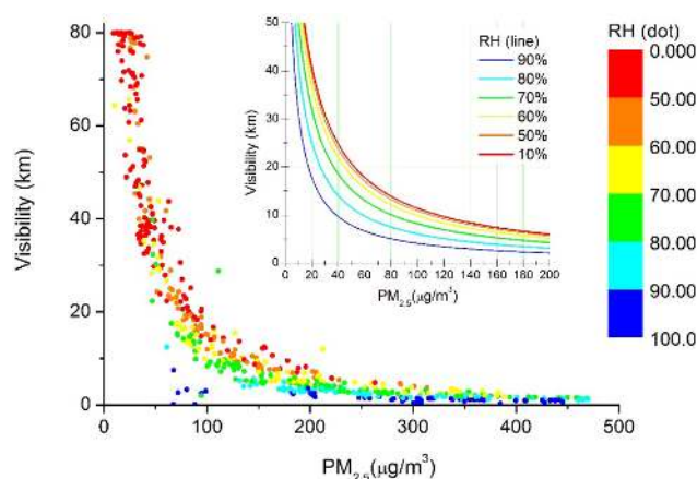
Figure 15. Variation of visibility at different RH values and different concentrations of \text{PM}_{2.5} , observed (dots) and simulated (lines).
