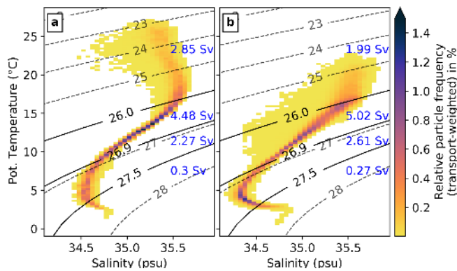
Figure 5. \theta S diagram of Agulhas leakage for experiment P (a) in the Agulhas Current at 32° S and (b) at the first crossing of the Good Hope section. The relative transport-weighted particle frequency is shown per 0.25^{\circ}\text{C} \times 0.05 psu bin in percent. Potential density levels used to separate upper, central, intermediate and deep waters are highlighted by solid black lines, and blue numbers indicate the transport of these water masses.
