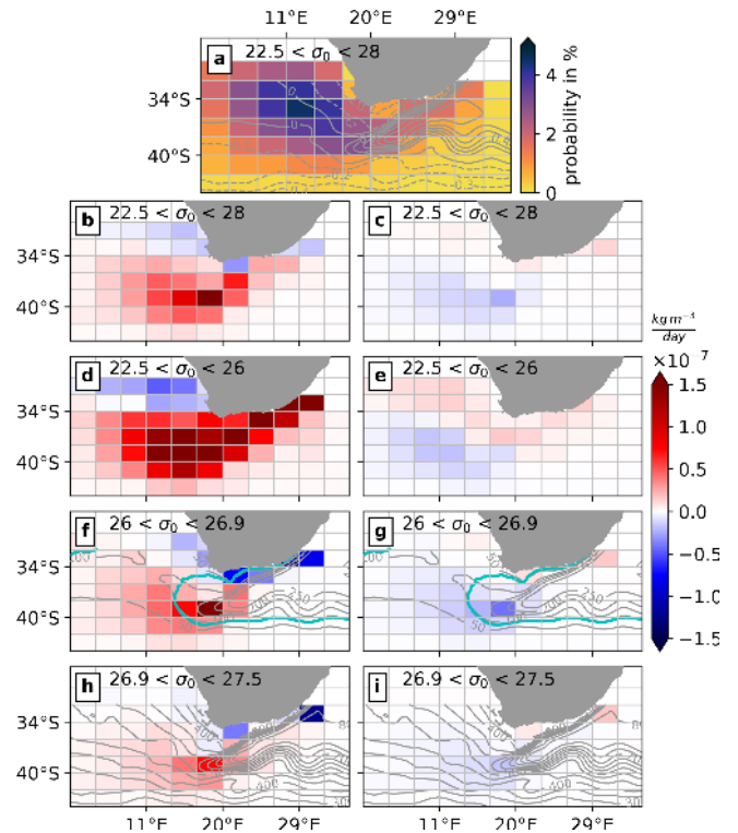
Figure 7. Pathways and horizontal distribution of the density changes of Agulhas leakage for experiment P: (a) relative transport-weighted probability in percent of all Agulhas leakage waters (considering all Agulhas leakage particles per bin at each time step). Contour lines show the mean (1958–2014) sea surface height (in m). Density changes due to the (b, d, f, h) thermal and (c, e, g, i) haline effect for (b, c) all water masses, (d, e) upper waters ( 22.5 < \sigma_0 < 26 ), (f, g) central waters ( 26 < \sigma_0 < 26.9 ) and (h, i) AAIW ( 26.9 < \sigma_0 < 27.5 ). To assign waters to these water masses, \sigma_0 in the Agulhas Current at 32^\circ\text{S} is used. The bin size of all histograms is 2^\circ in latitude \times 3^\circ in longitude. See Sect. 2.3 for details on the calculation. Grey contour lines in (f, g) and (h, i) show the mean (1958–2014) depth of the \sigma_0 = 26 and \sigma_0 = 26.9 surfaces, respectively. East of the cyan line the mean (1958–2014) depth of \sigma_0 = 26 is below the mean (1958–2014) winter (JJA) mixed layer depth.
