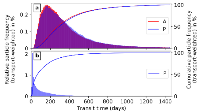
Figure 3. Mean (1958–2014) transit time distribution (transport-weighted) of Agulhas leakage from the Agulhas Current at 32^\circ S to (a) the Good Hope section and (b) 20^\circ E for experiment A in red and P in blue, overlapping probabilities are shown in purple. The transit time to 20^\circ E can not be analysed in experiment A because it was run in the quantitative mode of Ariane.
