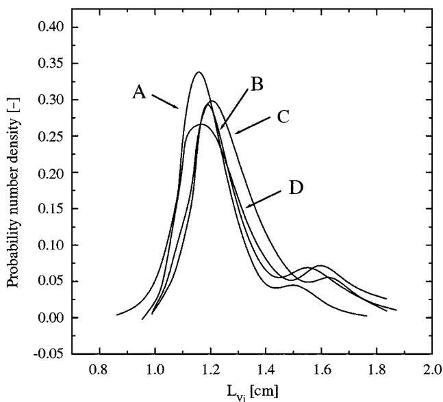
Fig. 2. Probability density of bubble chord length in gas-liquid countercurrent bubble column bioreactors( U_G=0.03 m/s, U_L=0.01 m/s). A B C D Bubble distribution mode: Even Wall-side Central Asymmetric
