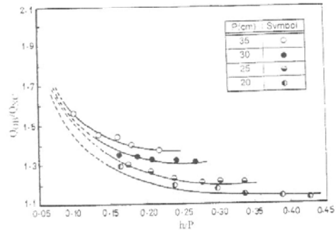
Fig.(24). Variation of ( Q_{nc}/Q_{ss} ) with ( h/P ) for oblique weirs of crest radius ( R ) =10cm and ( \alpha )=30°.
