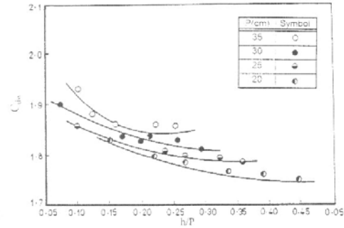
Fig. (12), Variation of ( C_{dw} ) with ( h/P ) for oblique weirs of crest radius ( R ) = 10cm and ( \alpha )=45°.
