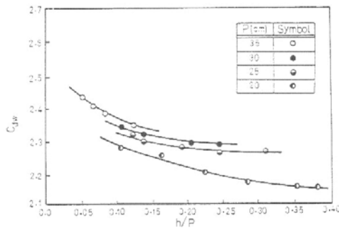
Fig. (7), Variation of ( C_{dw} ) with ( h/P ) for oblique weirs of crest radius ( R ) = 5cm and ( \alpha )=60°.
