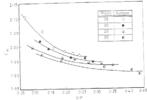
Fig. (10), Variation of ( C_{dw} ) with ( h/P ) for oblique weirs of crest radius ( R )=7.5cm and ( \alpha )=60°.
