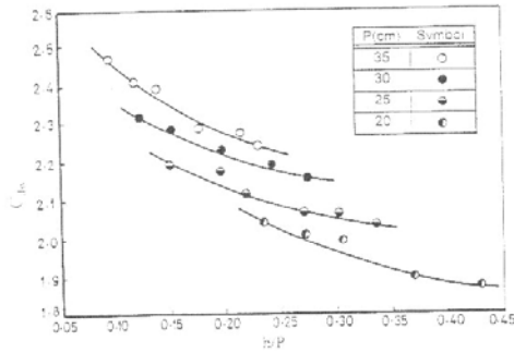
Fig. (9), Variation of ( C_{dw} ) with ( h/P ) for oblique weirs of crest radius ( R ) =7.5cm and ( \alpha )=45°.
