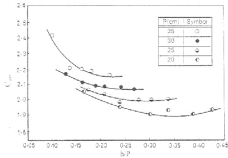
Fig. (11), Variation of ( C_{dw} ) with ( h/P ) for oblique weirs of crest radius ( R )=10cm and ( \alpha )=30°.
