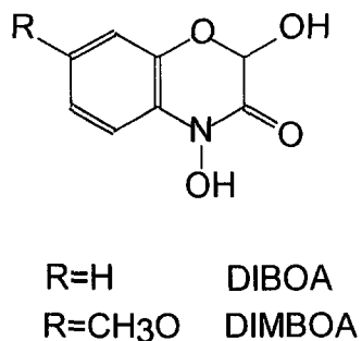
FIG. 1. Chemical structures of DIMBOA (2,4-dihydroxy-7-methoxy-1,4-benzoxazin-3-one) and DIBOA (2,4-dihydroxy-1,4-benzoxazin-3-one), the main hydroxamic acid aglucones present in wheat extracts.
