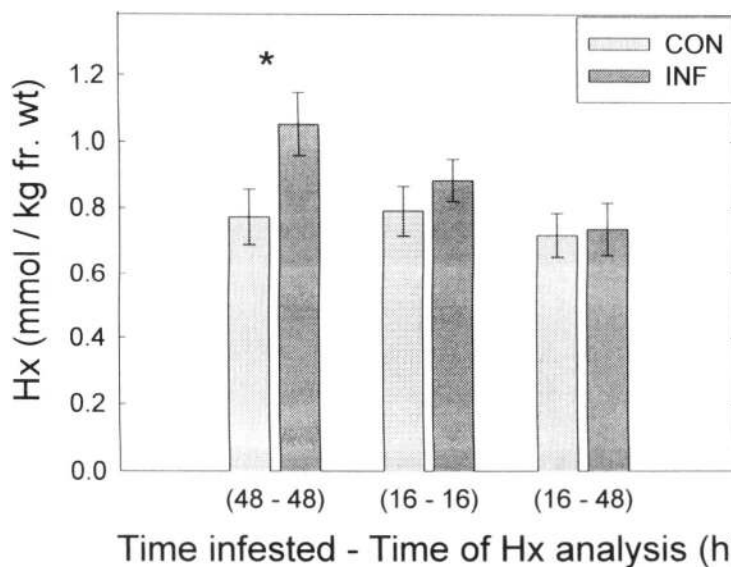
FIG. 3. Hydroxamic acid (Hx) content (mean \pm SE, eight replicates) of the primary leaf of aphid-infested (20 individuals) (INF) and noninfested control (CON) seedlings of wheat after different duration of infestation and time elapsed to Hx analysis since the onset of infestation. *Significant differences between control and infested plants at P < 0.05 (one-way ANOVA).
