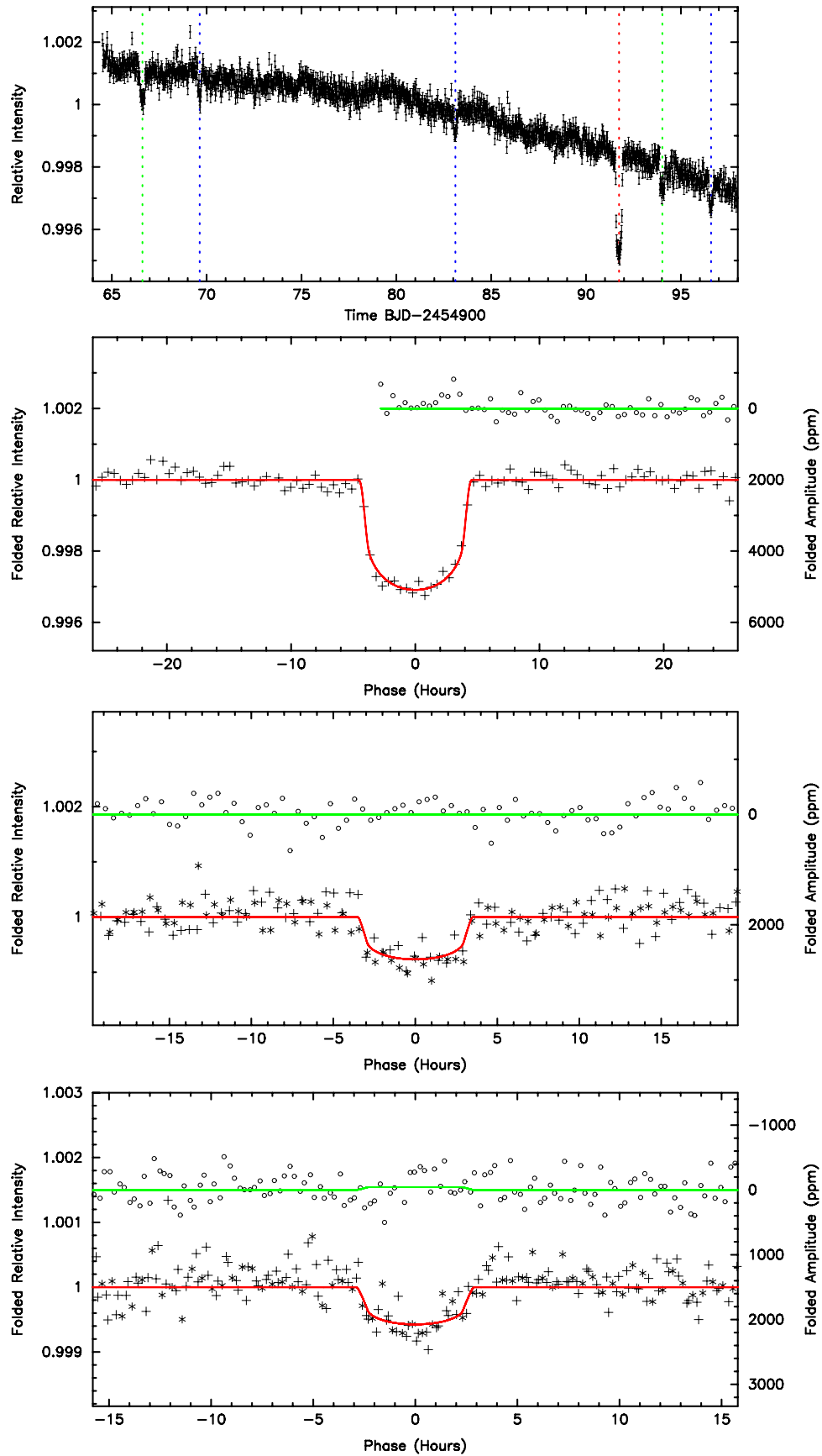
Figure 11. Three candidate planets associated with KIC 8394721. The position of the vertical dotted lines shows the position of the transits observed for each of the candidates.
