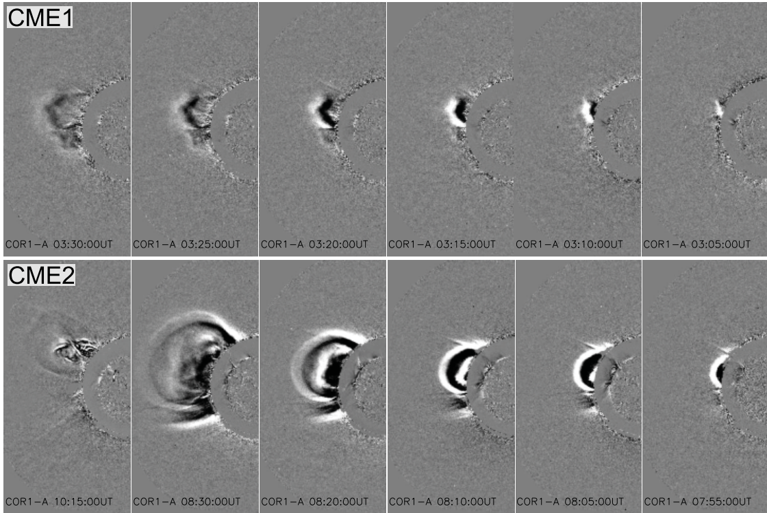
Fig. 2.— CME1 and CME2 in EUV and white light observations. Top : Sequence of EUVI/COR1 STEREO-A running difference images of CME1. Bottom : Sequence of EUVI/COR1 STEREO-A running difference images of CME2.
