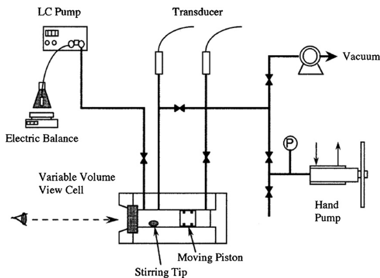
Figure 7 Schematic representation of the scrPE apparatus.
