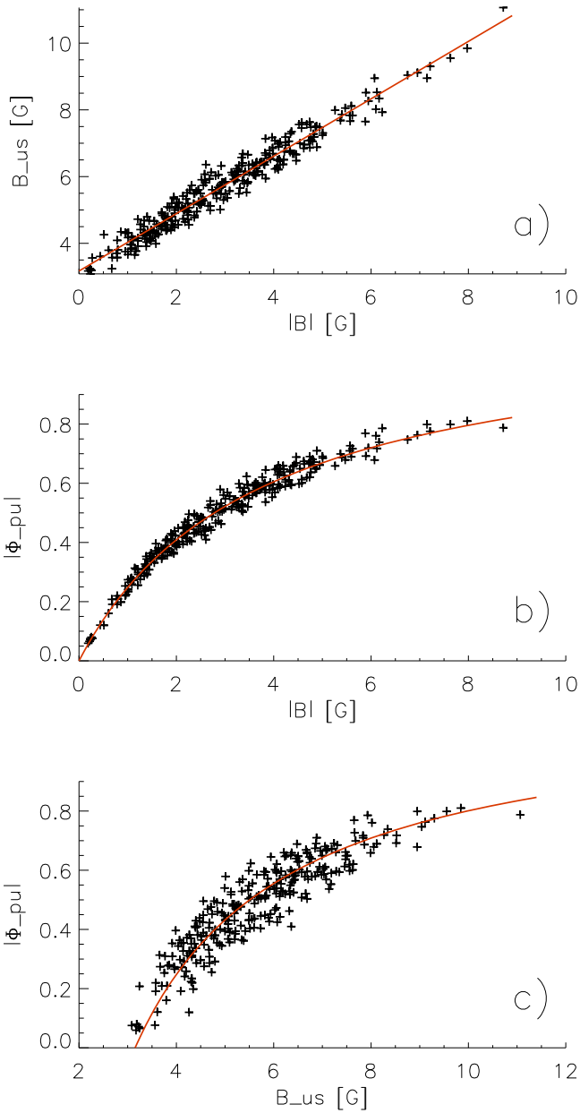
Figure 6. Scatter plots of the mean unsigned magnetic field densities vs. the mean magnetic field densities (a), the percentage unbalanced magnetic flux vs. the mean magnetic field densities (b), and the percentage unbalanced magnetic flux vs. the mean unsigned magnetic field densities (c), derived from all coronal holes. The corresponding fits given by Equations (19)–(21) are over-plotted in red.
