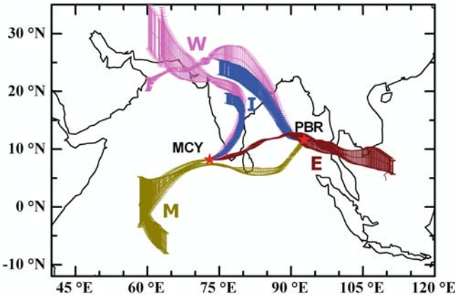
Figure 9. Back trajectory groups arriving at the 1800 m sl over MCY and PBR for the month of April. The vertical bars over the mean line show the spatial spread of each group. Details of grouping the trajectories are given in the text and table 2.
