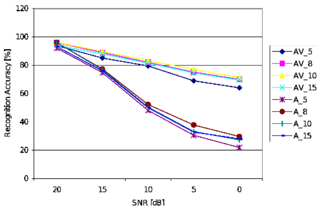
Fig. 6. Recognition results of audio and audio-visual speech, with varying degrees of noisy audio signal and different numbers of states (numbers with names indicate the number of used states of HMM and CHMM)
