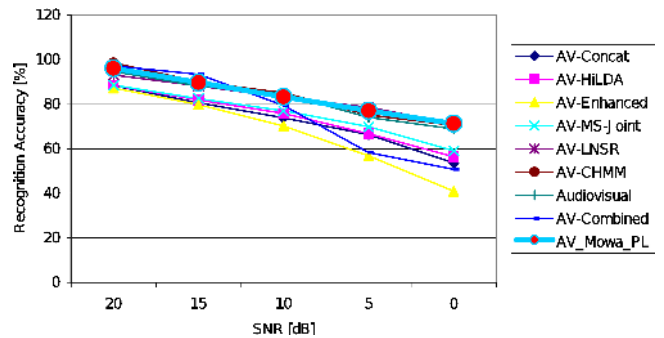
Fig. 7. The results of comparing the level of recognition errors of audio-visual speech for different methods
