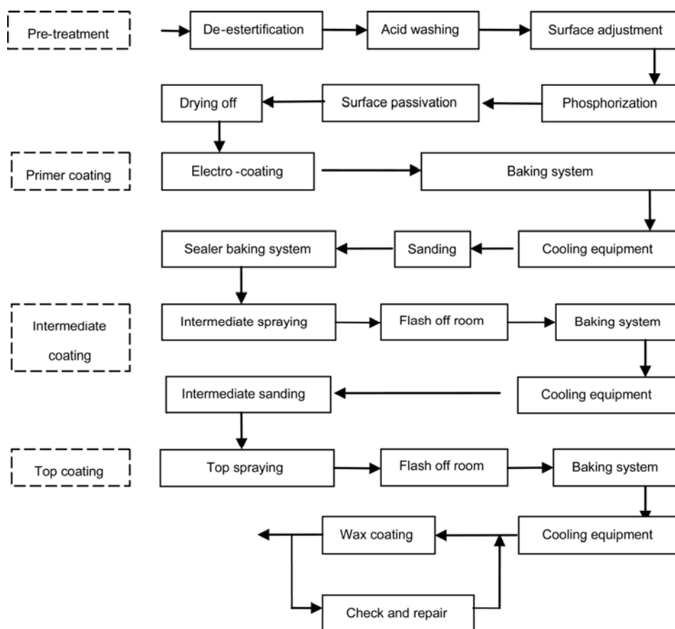
Figure 1 Process flow chart of a typical automobile manufacturing enterprise.
