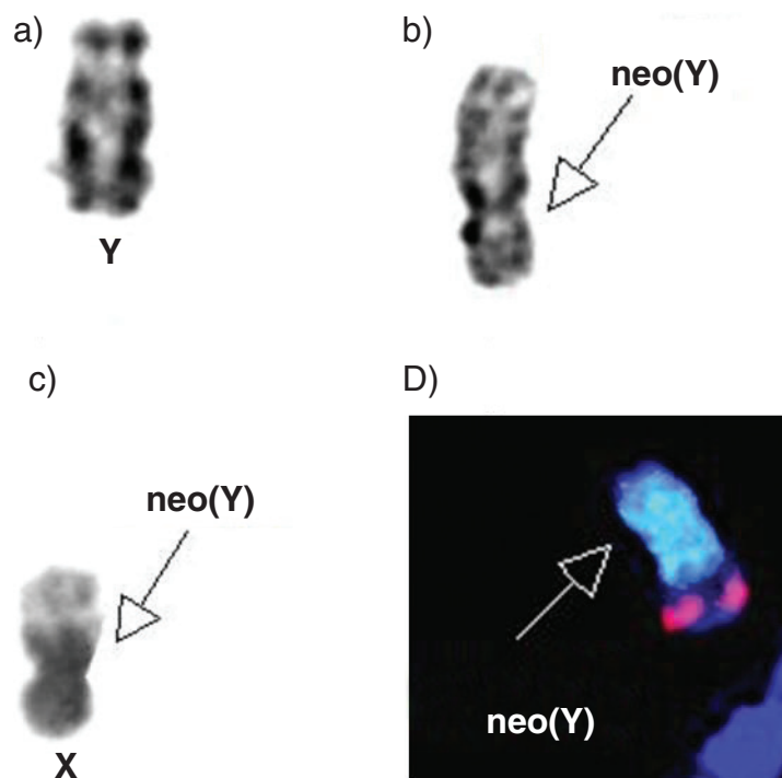
FIG. 2 Representative images showing a normal Y chromosome (a), a neocentromere of a Y chromosome (b), and C-banding and FISH indicating the marker was a neocentromere of the Y chromosome (c) and (d).
