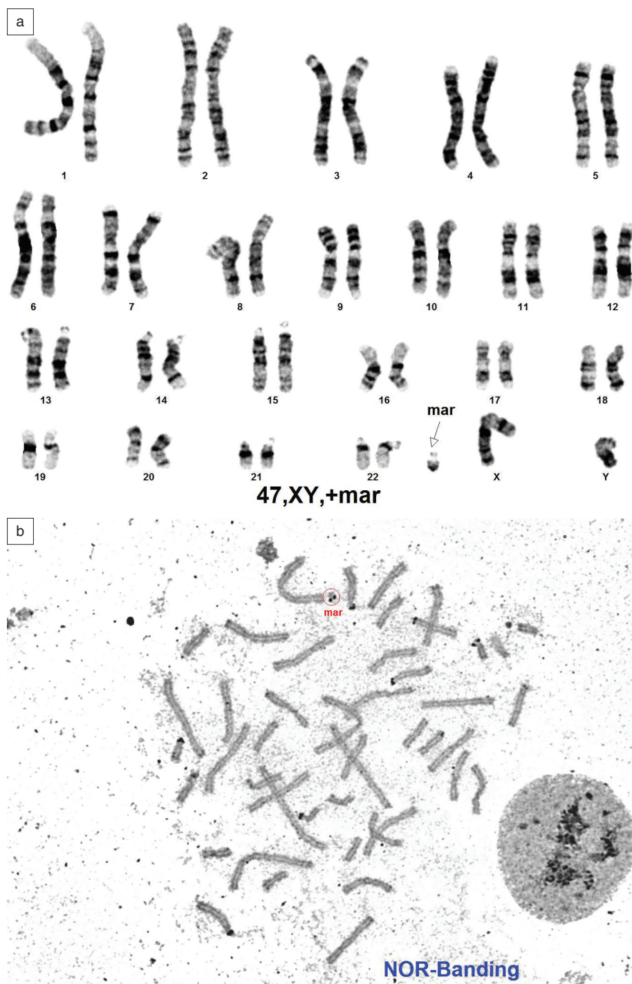
FIG. 1 Representative images showing GTG-banding of a marker chromosome (a) and NOR-banding with an acrocentric origin of a marker (b).
