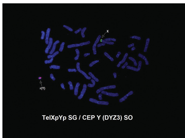
FIG. 3 Representative FISH images with Tel Xp/Yp SpectrumGreen and CEP Y (DYZ3) showing the marker was a ring Y chromosome.
