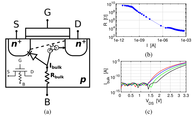
Fig. 11. (a) Cross-Section and schematic representation of the cause of kink effect at 4 K; (b) N-well resistance versus current at 4 K; the resistance value at 300 K is 3.5 k \Omega ; (c) I_{bulk}(V_{DS}) of thick-oxide NMOS, W/L = 2.32/0.322 at 4 K.
