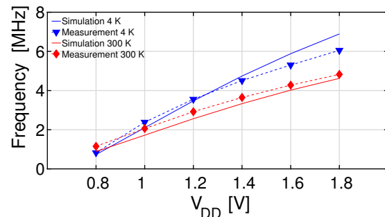
Fig. 17. Ring oscillator frequency versus supply voltage ( V_{DD} ) at 300 K and 4 K. Measurements (dotted lines) and simulations (solid lines) are compared with the compact model presented in Section IV.
