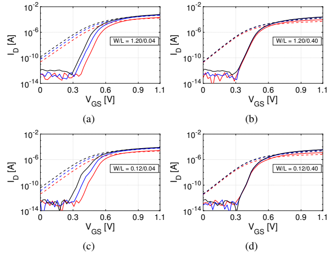
Fig. 6. Measured I_D(V_{GS}) characteristics of thin-oxide NMOS in 40-nm CMOS. V_{DS} = [0.1 \text{ V}; 0.6 \text{ V}; 1.1 \text{ V}] . Solid line: 4 K; dashed line: 300 K.
