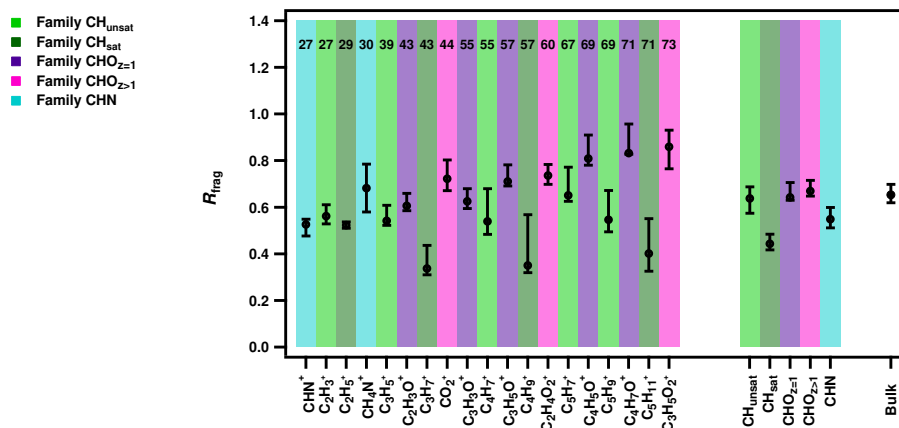
Figure 5. Median recovery of single organic fragments, and chemical families for the Zurich spring campaign (offline vs. online PM 2.5 AMS). The first and third quartiles of the inter-sample variability are shown as error bars. A ratio of 1 indicates a recovery of 100%. The fragments are color-coded with the family (CH (hydrocarbon fragments, split into saturated and unsaturated), CHO z=1 and CHO z>1 (oxygenated fragments), and CHN, nitrogen-containing hydrocarbon fragments). Numbers across the top of the plot indicate the fragments' nominal mass. Families include all respective fragments weighted by their mass contribution.
