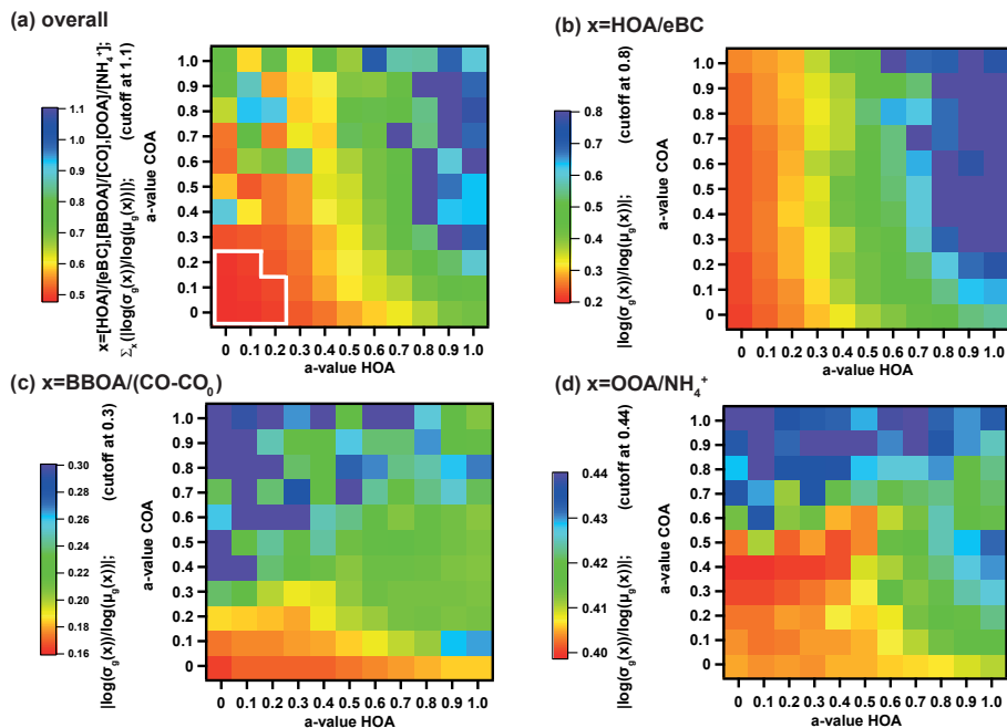
Figure 8. Relative width of the distributions ( c_j/c_{\text{marker}} ) displayed as a function of a_{\text{HOA}} and a_{\text{COA}} . Panel (a) shows the sum of the criteria for HOA, BBOA, and OOA being the sum of OOA1 and OOA2. (The chosen solutions are pointed out in the white area.) Panels (b–d) show the individual criteria as a function of the a values of HOA and COA a_{\text{HOA}} , a_{\text{COA}} .
