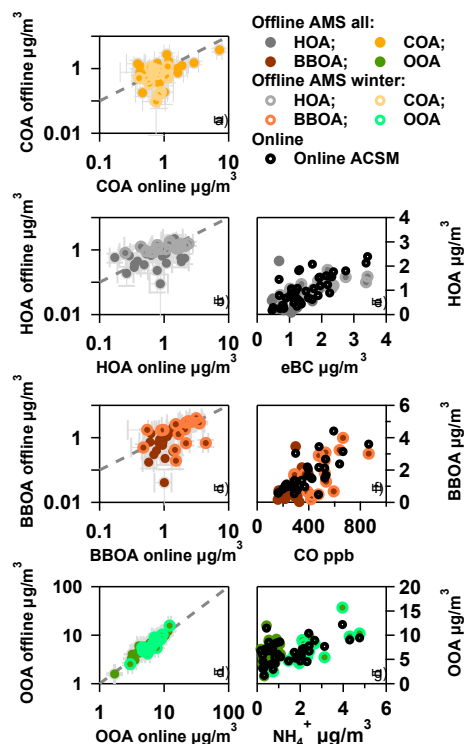
Figure 11. Comparison of factor contributions from separate offline ( PM_{10} AMS, two constrained factors: HOA, COA) and online ( PM_1 ACSM) source apportionment using ME-2 (traffic (HOA), cooking (COA), biomass burning (BBOA), and oxygenated organic aerosol; OOA = OOA1 + OOA2 ). Factor-specific recoveries ( R_k ) are applied to the offline contributions. Error bars (in gray) denote the variability between the different ME-2 solutions and for different recorded spectra per sample for offline and for online only the first of the two. Panels (a–d) show scatter plots comparing the absolute contribution of the respective source/OA category for offline AMS and online ACSM measurements. The color code distinguishes all factor contributions (bullets, saturated colors) from winter points (open circle, light colors). The gray dashed line indicates the 1 : 1 line. Panels (e–g) show the correlation with the respective markers: black symbols represent the absolute contribution of the respective source for the online ACSM measurements and the colored symbols represent the absolute contribution of the same source for the offline AMS measurements.
