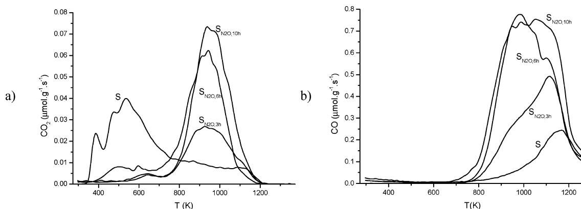
Figure 2. TPD spectra for the samples oxidized in 50% N 2 O in N 2 : (a) CO 2 evolution; (b) CO evolution.
