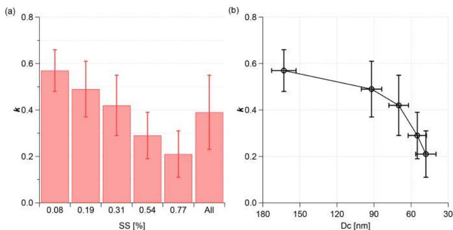
Figure 9. (a) Derived \kappa values at different supersaturations. (b) \kappa values as a function of the corresponding d_{crit} . Error bar represents the 1 standard deviation.
