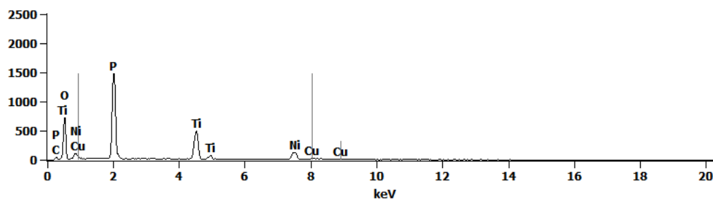
Fig. 6. EDS of NiTi surface after PEO treatment at 450 V for 3 minutes in the electrolyte consisting of 300 g \text{Cu}(\text{NO}_3)_2 in 1 L \text{H}_3\text{PO}_4 ( \text{Cu wt}\%/ \text{P wt}\% = 0.13 ; \text{Cu at}\%/ \text{P at}\% = 0.06 )
