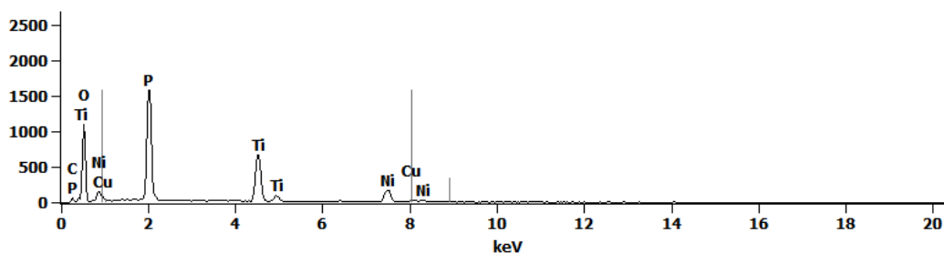
Fig. 8. EDS of NiTi surface after PEO treatment at 450 V for 3 minutes in the electrolyte consisting of 600 g \text{Cu}(\text{NO}_3)_2 in 1 L \text{H}_3\text{PO}_4 ( \text{Cu wt\%/P wt\%} = 0.19 ; \text{Cu at\%/P at\%} = 0.09 )
