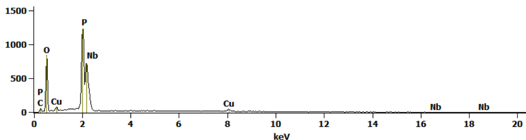
Fig. 4. EDS spectrum of Niobium after PEO treatment at 450 V for 3 minutes in the electrolyte consisting of 600 g \text{Cu}(\text{NO}_3)_2 in 1 L \text{H}_3\text{PO}_4 ( \text{Cu wt\%/P wt\%} = 0.22 ; \text{Cu at\%/P at\%} = 0.11 )
