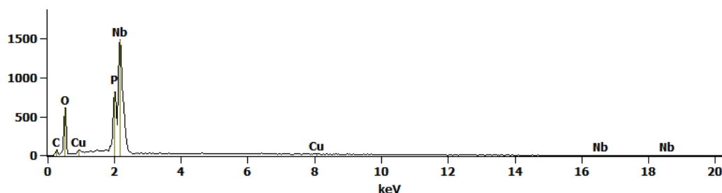
Fig. 2. EDS spectrum of Niobium after PEO treatment at 450 V for 3 minutes in the electrolyte consisting of 300 g \text{Cu}(\text{NO}_3)_2 in 1 L \text{H}_3\text{PO}_4 ( \text{Cu wt\%/P wt\%} = 0.16 ; \text{Cu at\%/P at\%} = 0.08 )
