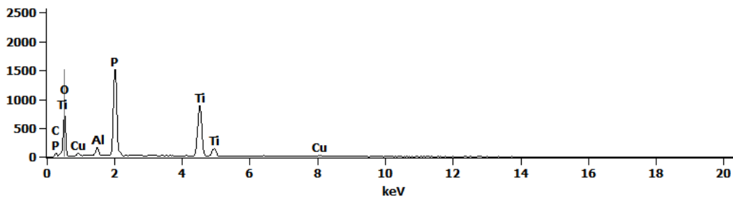
Fig. 10. EDS of Ti6Al4V surface after PEO treatment at 450 V for 3 minutes in the electrolyte consisting of 300 g \text{Cu}(\text{NO}_3)_2 in 1 L \text{H}_3\text{PO}_4 (Cu wt%/P wt% = 0.12; Cu at%/P at% = 0.06)
