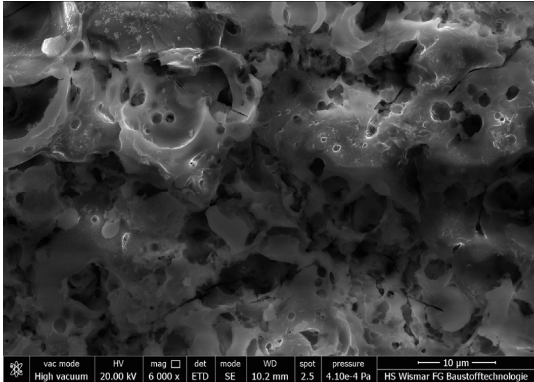
Fig. 9. SEM image of Ti6Al4V surface after PEO treatment at 450 V for 3 minutes in the electrolyte consisting of 300 g \text{Cu}(\text{NO}_3)_2 in 1 L \text{H}_3\text{PO}_4
