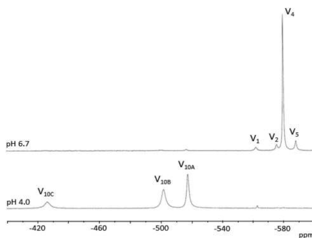
Fig. 2 51 V NMR (105.2 MHz, 9.4 T) spectra, at ambient temperature of 50 mM (total vanadium) concentration of decavanadate (pH 4.0) (A) and metavanadate solutions (pH 6.7) (B). All spectra were acquired in the presence of 10% D 2 O. V 10A , V 10B and V 10C represent signals of vanadium sites in V 10 . The 51 V NMR V 1 signals correspond to the orthovanadate species namely, monomeric vanadate (VO 4 3- , HVO 4 2- and H 2 VO 4 - ), whereas the metavanadate species includes dimeric V 2 (HV 2 O 7 3- and H 2 V 2 O 7 2- ), regardless of the state of protonation, V 4 and V 5 , that corresponds to cyclic tetrameric ([V 4 O 12 ] 4- ) and pentameric vanadate ([V 5 O 15 ] 5- ), respectively.
