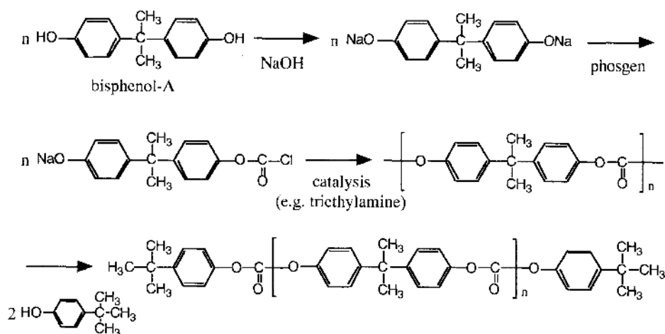
Scheme 1. Solvent method.
