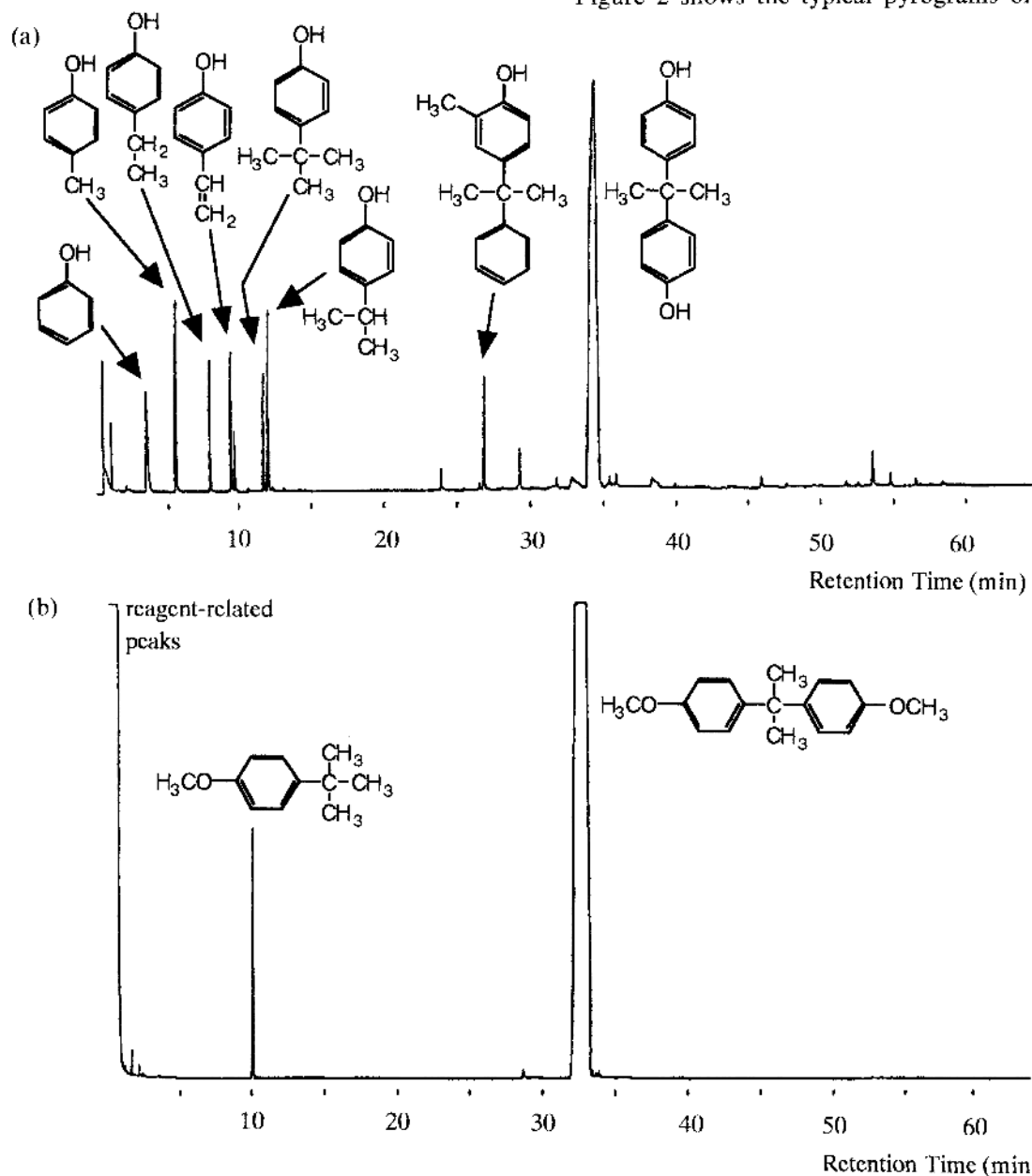
Figure 2 Pyrograms of SM-PC: (a) a raw SM-PC observed by conventional pyrolysis at 600°C and (b) a fractionated SM-PC (S-2) observed by reactive pyrolysis at 400°C in the presence of TMAH.
