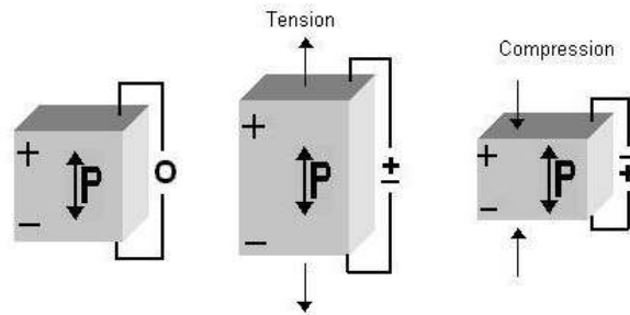
Figure 2.18. Direct Piezoelectric Effect (from Boston Piezo-Optics, Inc.)
