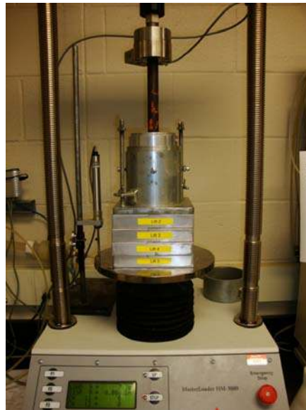
Figure 4.3. Static Undercompaction of Specimens
