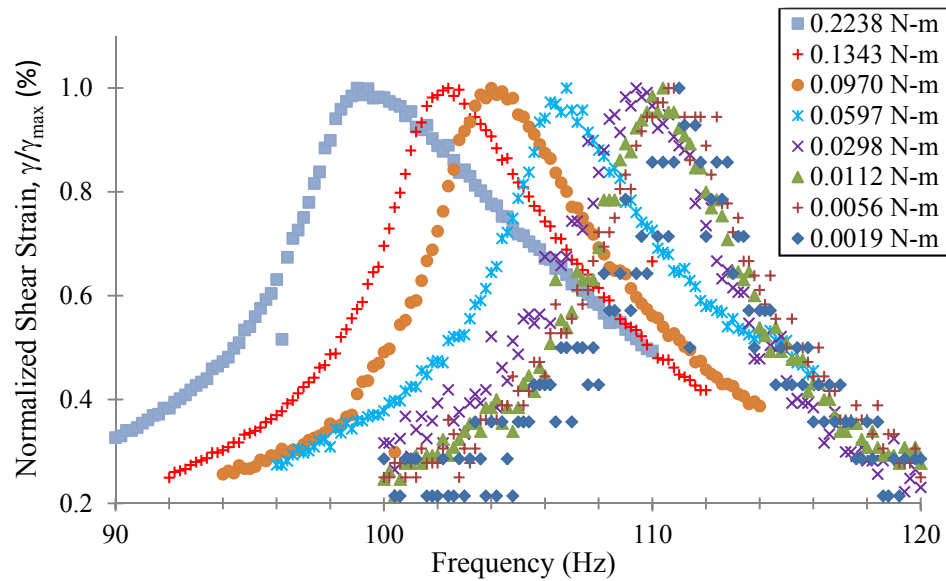
Figure 6.2. Normalized Frequency Response Curve (98.5% Kaolin : 1.5% EPS Specimen G @ \sigma_{\text{cell}} = 25\text{kPa} )
