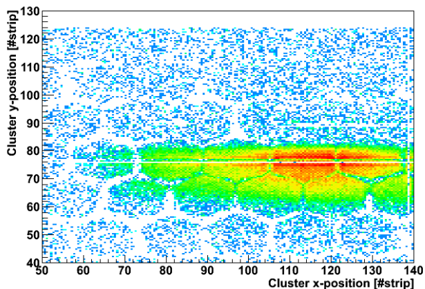
Fig. 12. Reconstructed cluster positions in the subregions near the beam spot of two different honeycomb triple-GEM configurations.
