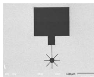
FIGURE 6. SEM image of patterned device
