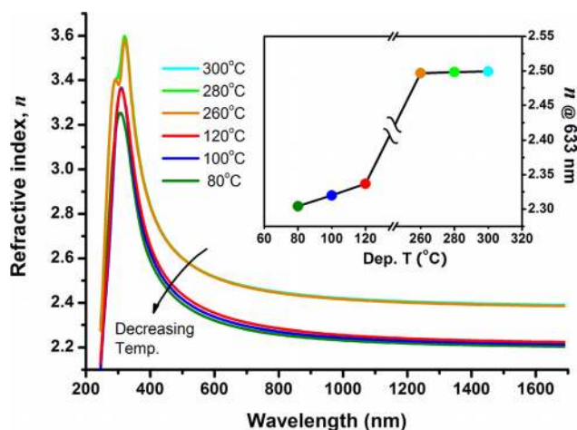
Fig. 5. (Color online) Refractive index spectra of ALD TiO 2 films deposited at temperatures between 300 and 80 °C obtained by spectroscopic ellipsometry. The inset shows the values at 633 nm.
