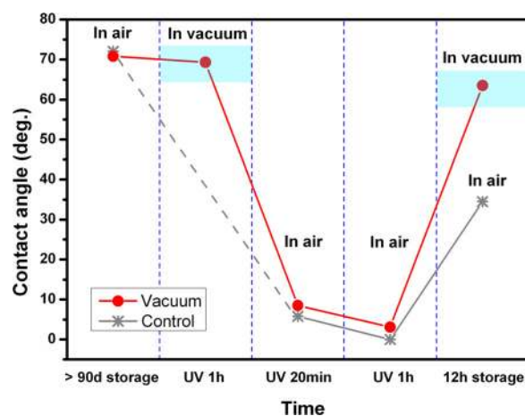
FIG. 11. (Color online) Comparison of water contact angles of samples treated in vacuum and in air.
