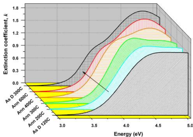
FIG. 7. (Color online) Extinction coefficient spectra of different ALD TiO 2 films. Samples from bottom to top: as deposit at 120 °C; 120 °C deposited and annealed at 200, 300, 400, and 600 °C; as deposit at 300 °C.
