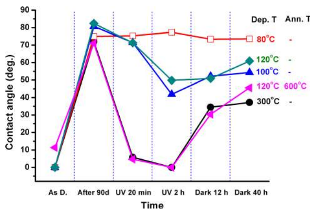
FIG. 9. (Color online) Evolution of water contact angles of different ALD TiO 2 films vs storage time and UV illumination.
