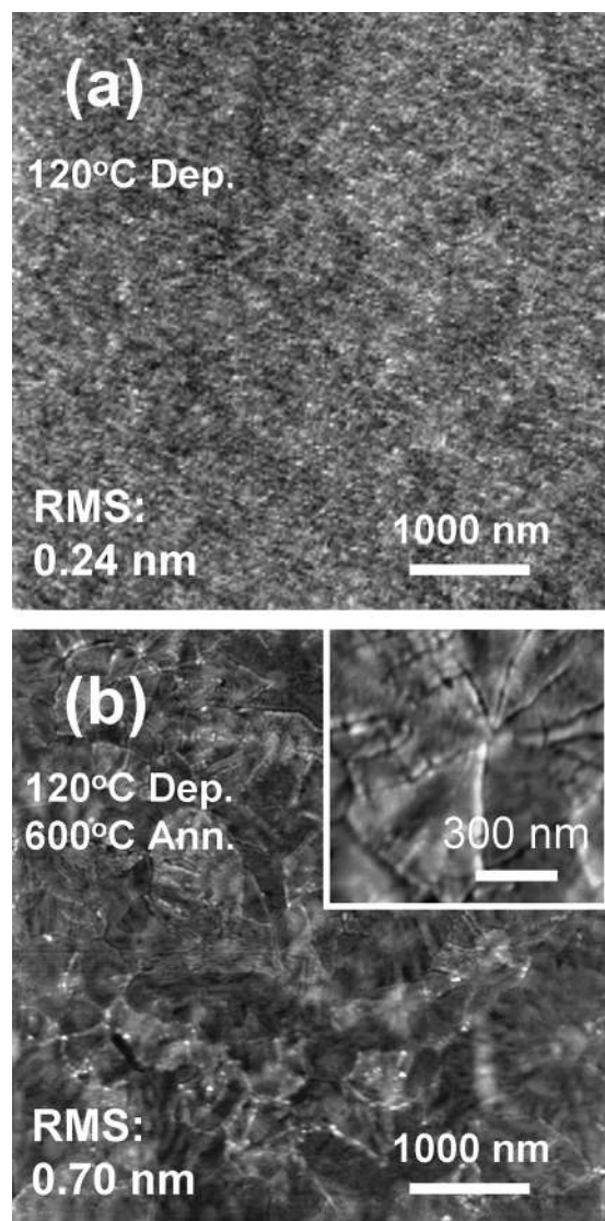
FIG. 2. AFM images of ALD TiO 2 films deposited at 120 °C: (a) as-deposited and (b) after annealing. A closeup of the recrystallized structure is shown in the inset.
