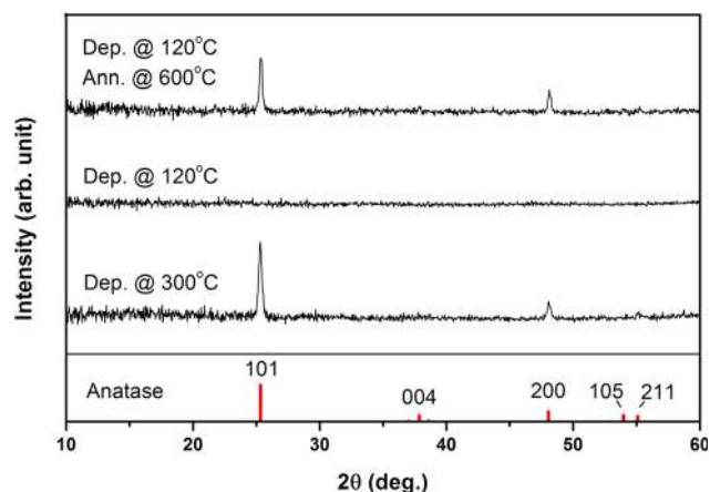
FIG. 3. (Color online) X-ray diffraction spectra of as-deposited and annealed ALD TiO 2 films. Diffraction peaks of anatase TiO 2 are also indicated.
