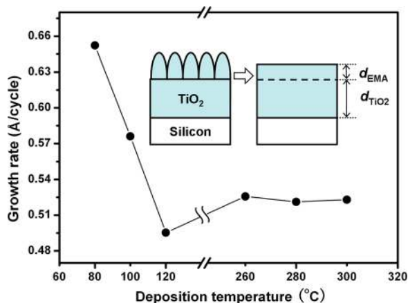
Fig. 4. (Color online) Growth rate of ALD TiO 2 films deposited at high and low temperatures. The model with an EMA layer representing the roughness is also schematically shown.
