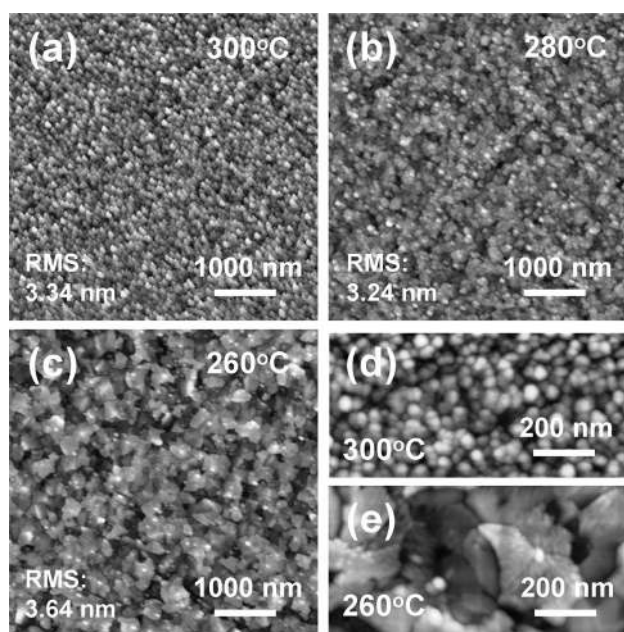
Fig. 1. AFM images of the surface morphology of ALD TiO 2 films deposited at (a) 300 °C, (b) 280 °C, and (c) 260 °C, together with grain size inspection of (d) the 300 °C sample and (e) the 260 °C sample.
