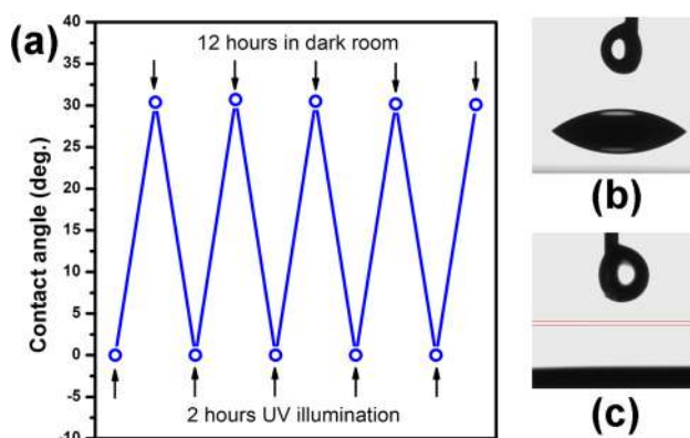
FIG. 10. (Color online) (a) Reversion of wettability of the 600 °C annealed sample under alternate UV illumination and storage in dark environment. [(b) and (c)] Representative photos of water drops in contact angle measurement.
