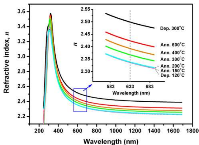
Fig. 6. (Color online) Recovering of refractive index for the 120 °C deposited samples by annealing. The annealing temperature ranges from 150 to 600 °C. For comparison, RI curves of the as-deposited 120 and 300 °C ALD TiO 2 films are also plotted.
