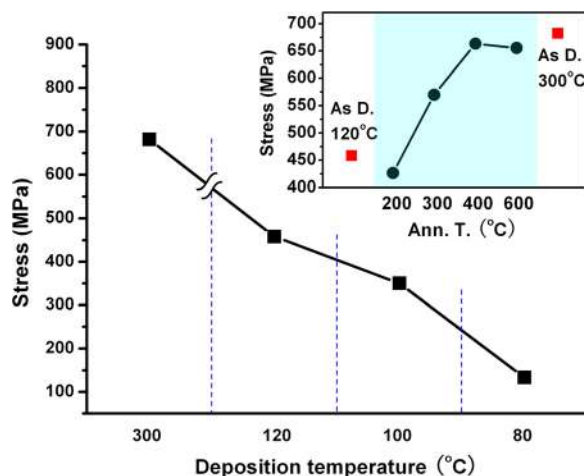
FIG. 8. (Color online) Relationship between the stress of ALD TiO 2 layers and their deposition temperature. The inset shows the effect of annealing on the stress of the 120 °C layers.
