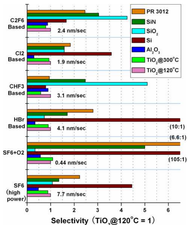
Fig. 12. (Color online) Etch rate diagram of ALD TiO 2 . The selectivity of frequently used materials, defined as the ratio of the etch rates of the materials over the etch rate of the 120 °C deposited TiO 2 , is plotted for different plasma etchants and conditions. The etch rate of the 120 °C deposited TiO 2 is listed next to the each corresponding recipe group.
