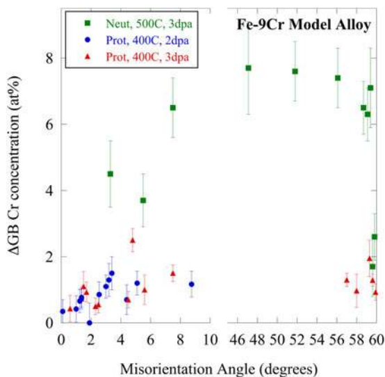
FIG. 3. Dependence of Cr RIS on grain boundary misorientation in Fe–9Cr model alloy irradiated with fast neutrons to 3 dpa at 500 °C, or with 2.0 MeV protons to 2–3 dpa at 400 °C. Note increasing RIS magnitudes with increasing misorientation for low-angle ( <10^\circ ) boundaries, and decreasing RIS magnitudes near \Sigma 3 grain boundaries ( 60^\circ ).
