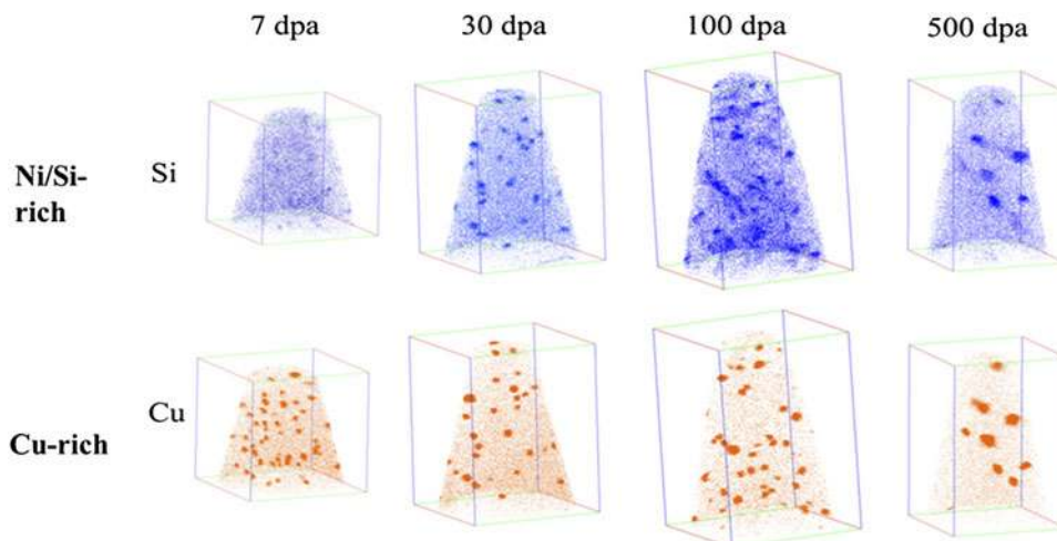
FIG. 17. Evolution of Ni/Si/Mn-rich and Cu-rich precipitates with dose in HCM12A following \text{Fe}^{++} irradiated at 400 °C.
