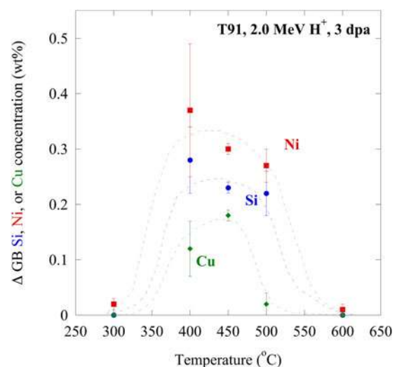
FIG. 2. Temperature dependence of Si, Ni, and Cu RIS in alloy T91 irradiated with 2.0 MeV protons to 3 dpa, showing enrichment between 400 and 500 °C and RIS suppression at 300 and 600 °C.
