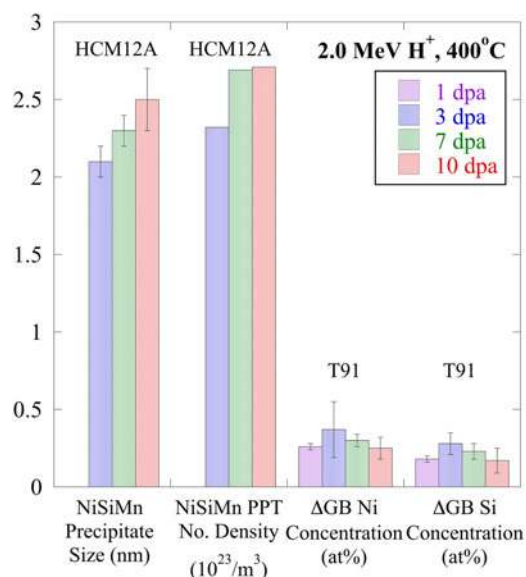
FIG. 10. Comparison of irradiation dose evolution of Ni–Si–Mn precipitates, and Ni and Si RIS in T91 and HCM12A irradiated with 2.0 MeV protons at 400 °C.
