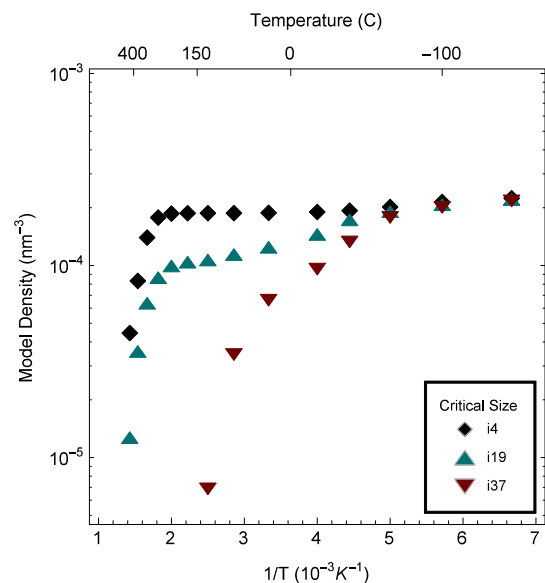
FIG. 27. Saturation density for each of the three thermal migration scenarios including induced motion for interstitial clusters with 4 or more members.
