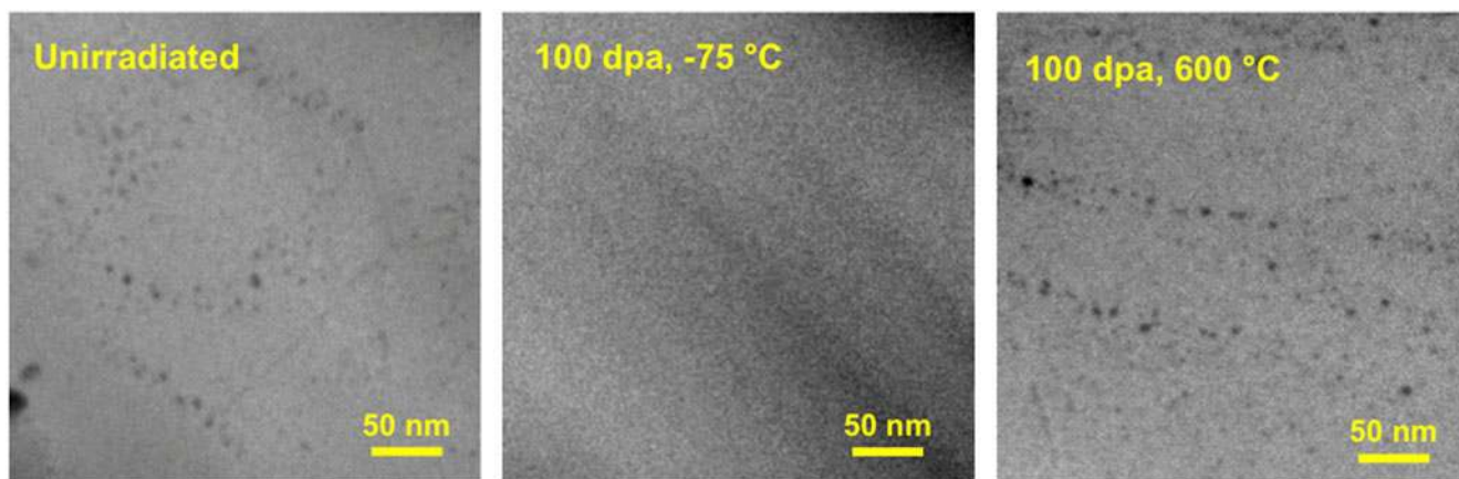
FIG. 19. Set of Fe–M jump-ratio images from a control 14YWT sample, and 14YWT samples irradiated to 100 dpa at temperatures ranging from –75 to 600 °C. The darker areas correspond to the nanoclusters.
