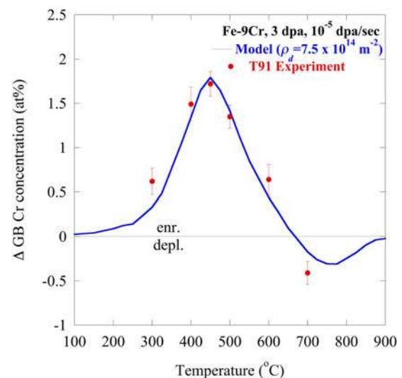
FIG. 6. Temperature dependence of IK modeled Cr RIS for Fe–9Cr, compared with experimental measurements from 2.0 MeV proton-irradiated T91, at 3 dpa, 10^{-5} dpa/s.
