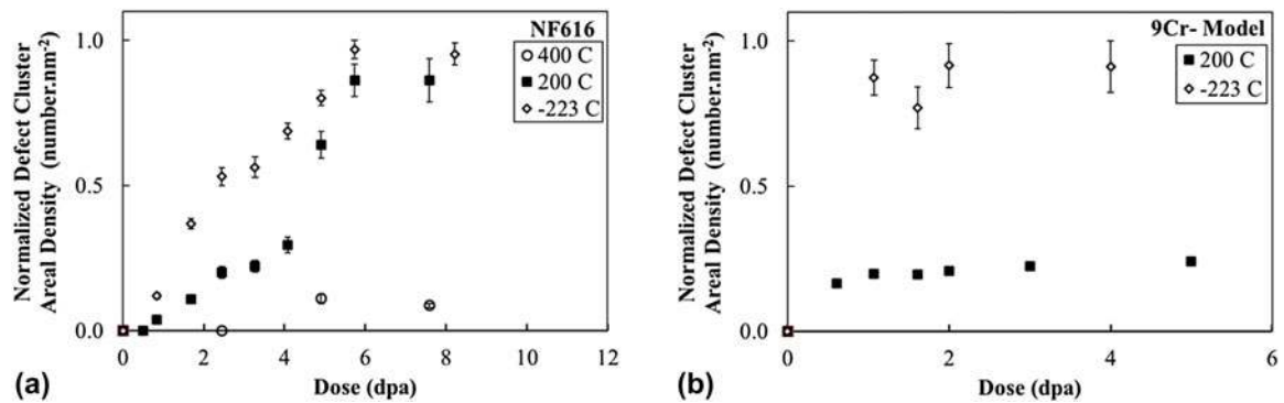
FIG. 24. Normalized defect cluster areal density of (a) NF616 and (b) 9Cr-model alloys as a function of dose. The defect cluster density is normalized to the highest value acquired (5.5 dpa at -223 °C for NF616 and 2 dpa at -223 °C for 9Cr-model alloy), plus the error bar. 89
