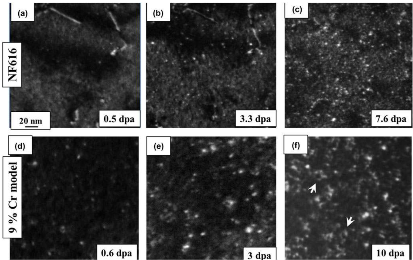
FIG. 22. Dark-field TEM images of microstructure evolution of NF616 under 1 MeV Kr irradiation at 200 °C.
