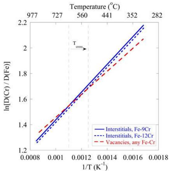
FIG. 7. Diffusion coefficient ratios of Cr to Fe for vacancies and interstitials in bcc Fe–Cr binary alloys. Crossover temperature, T_{cross} , decreases for increasing bulk Cr content. Below T_{cross} , Cr interstitial diffusion dominates, causing Cr enrichment. Above T_{cross} , Cr vacancy diffusion dominates, resulting in Cr depletion.
