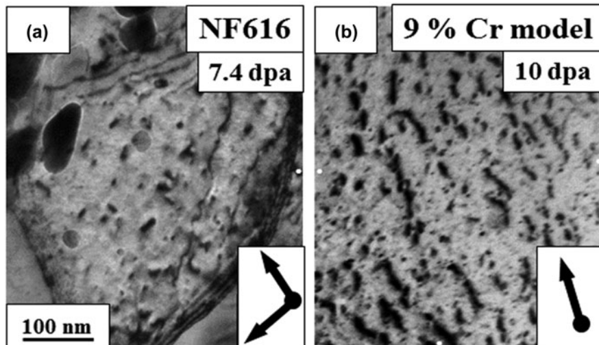
FIG. 23. Bright-field transmission electron micrographs of extended defects observed in NF616 and 9Cr-model alloys under 1 MeV Kr irradiations performed at 400 °C (a) and 25 °C (b), respectively. 89
