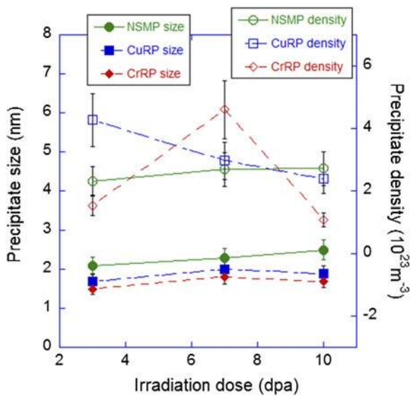
FIG. 12. Dose dependence of precipitate size and number density in HCM12A irradiated with 2 MeV protons at 400 °C.
