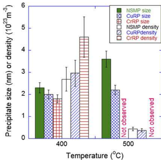
FIG. 13. Temperature dependence of precipitate size and number density in HCM12A irradiated with 2 MeV protons to 7 dpa.
