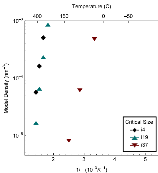
FIG. 26. Saturation density as a function of temperature for each of the three interstitial migration scenarios. The critical size refers to the smallest interstitial cluster which diffuses with a 1.3 eV activation energy.
