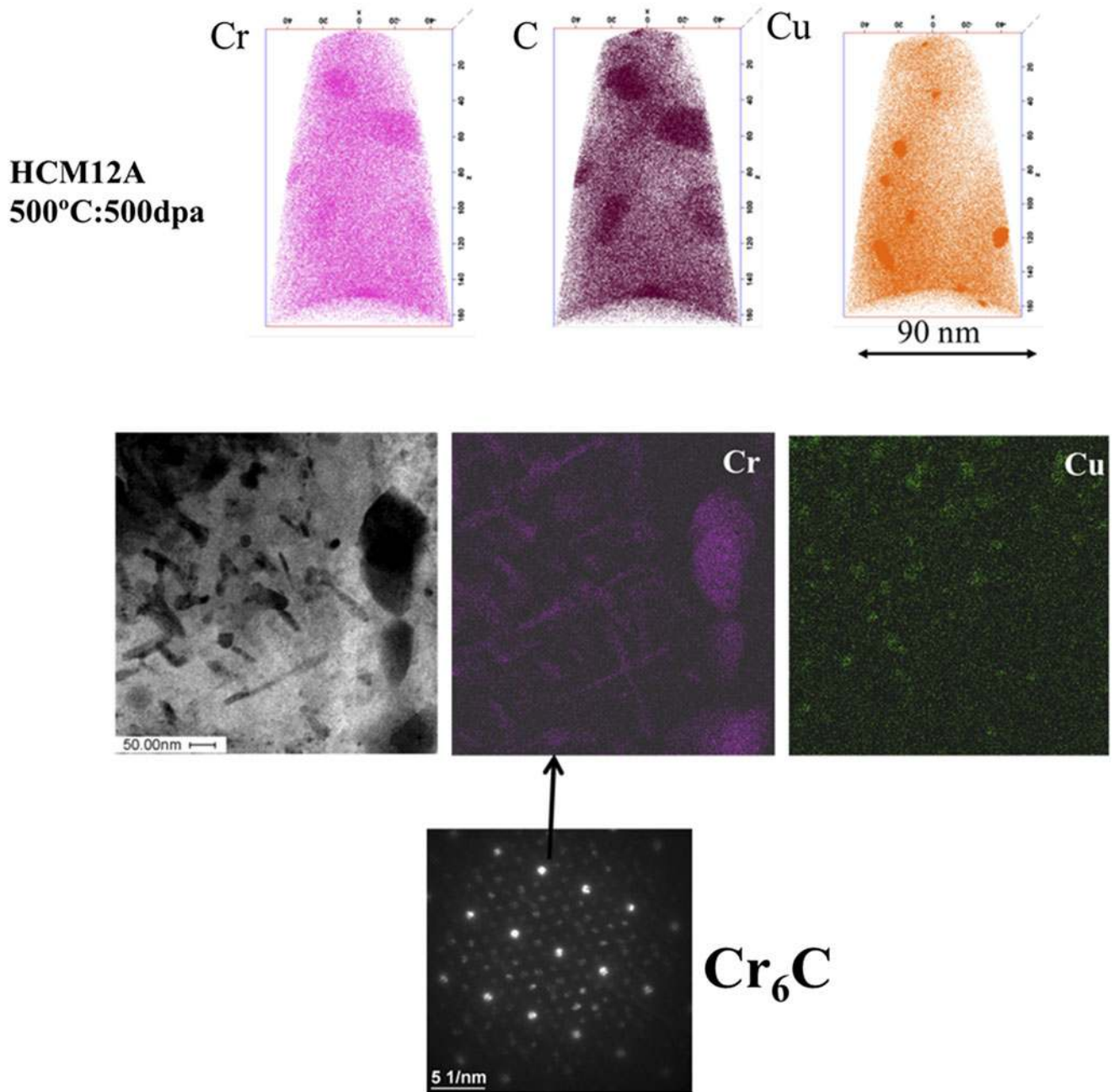
FIG. 18. Formation of \text{M}_6\text{C} carbides in HCM12A following \text{Fe}^{++} irradiation to 500 dpa at 500 °C.
