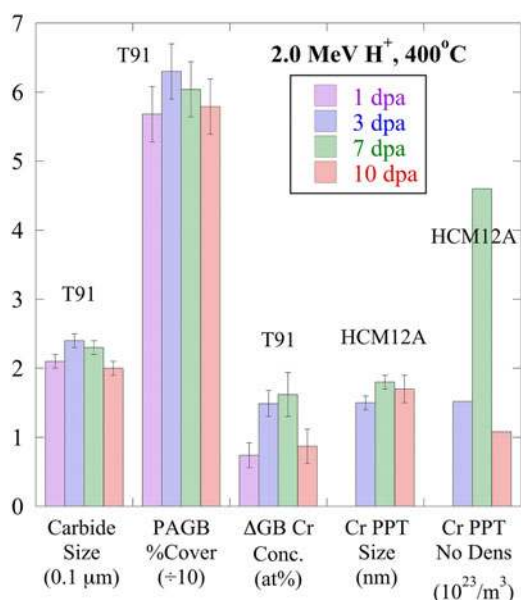
FIG. 9. Comparison of irradiation dose evolution of carbides, Cr RIS, and Cr-rich precipitates in T91 and HCM12A irradiated with 2.0 MeV protons at 400 °C.
