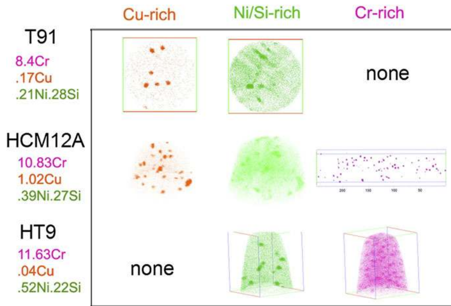
FIG. 15. Distribution of Cu-rich, Ni/Si/Mn-rich, and Cr-rich precipitates in T91, HCM12A, and HT-9 following irradiation to 7 dpa at 400 °C. The concentrations of Cr, Cu, Ni, and Si are also listed.
