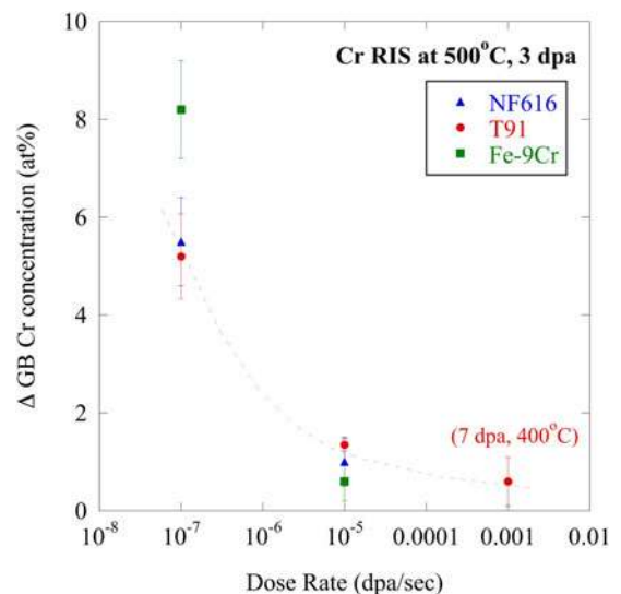
FIG. 4. Dependence of Cr RIS on irradiation dose rate for NF616 and T91 irradiated with fast neutrons ( \sim 10^{-7} dpa/s) and 2.0 MeV protons ( \sim 10^{-5} dpa/s) at 500 °C to 3 dpa, and with 5.0 MeV \text{Fe}^{++} ions ( \sim 10^{-3} dpa/s) at 400 °C to 7 dpa.
