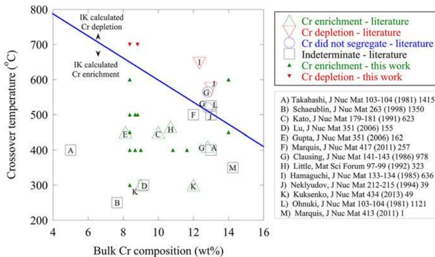
FIG. 8. Experimental measurements of the direction of Cr RIS in FM alloys, according to the literature (open symbols) and this work (closed symbols), as compared to the crossover temperature calculated in this work.
