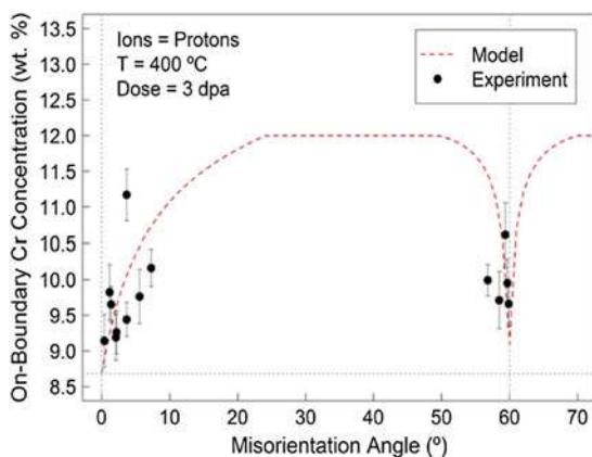
FIG. 5. Experimental (data points) and predicted (dashed line) grain boundary Cr concentration for a range of boundary misorientations under 3 dpa, 400 °C proton irradiation. Reprinted from Ref. 33.
