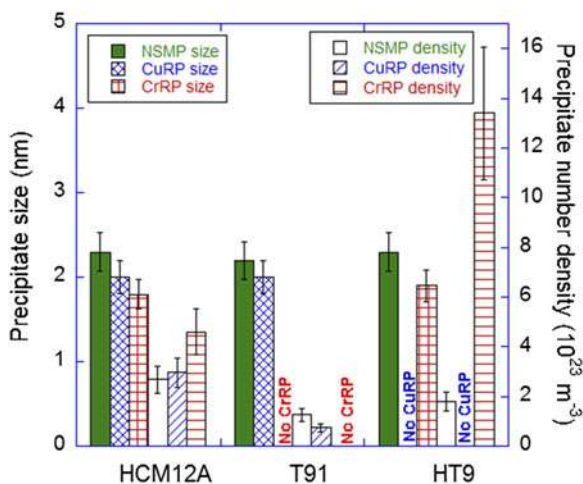
FIG. 14. Alloy dependence of precipitate size and number density following irradiation with 2 MeV protons to 7 dpa at 400 °C.
