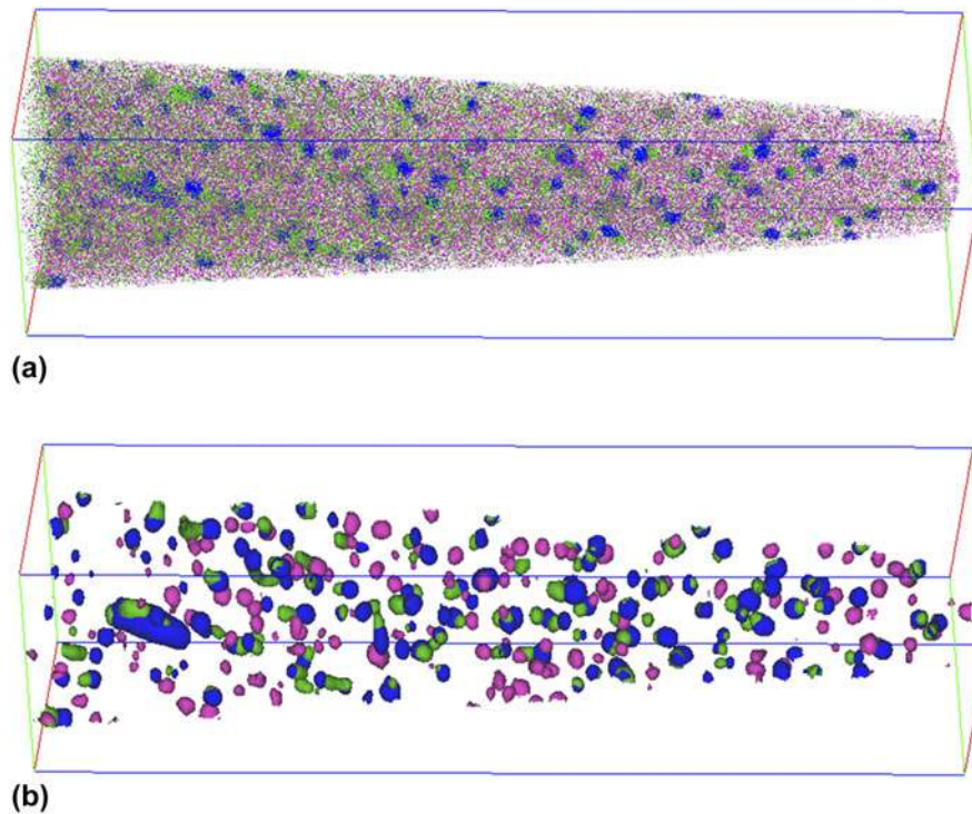
FIG. 11. APT image of a tip from HCM12A irradiated with 2 MeV protons to 7 dpa at 400 °C containing NSMPs, CuRPs, and CrRPs. (a) Ni (green), Cu (blue), and Cr (pink) atom maps. (b) NSMPs (green), CuRPs (blue), and CrRPs (pink) highlighted using isosurface plots. The dimensions of the box are 250 \times 63 \times 63 \text{ nm}^3 .
