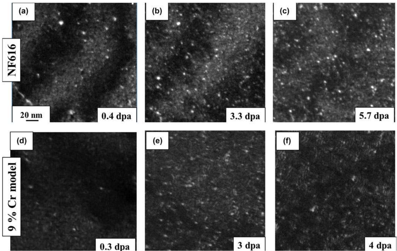
FIG. 21. Dark-field TEM images of microstructure evolution of NF616 under 1 MeV Kr irradiation at -223 °C.
