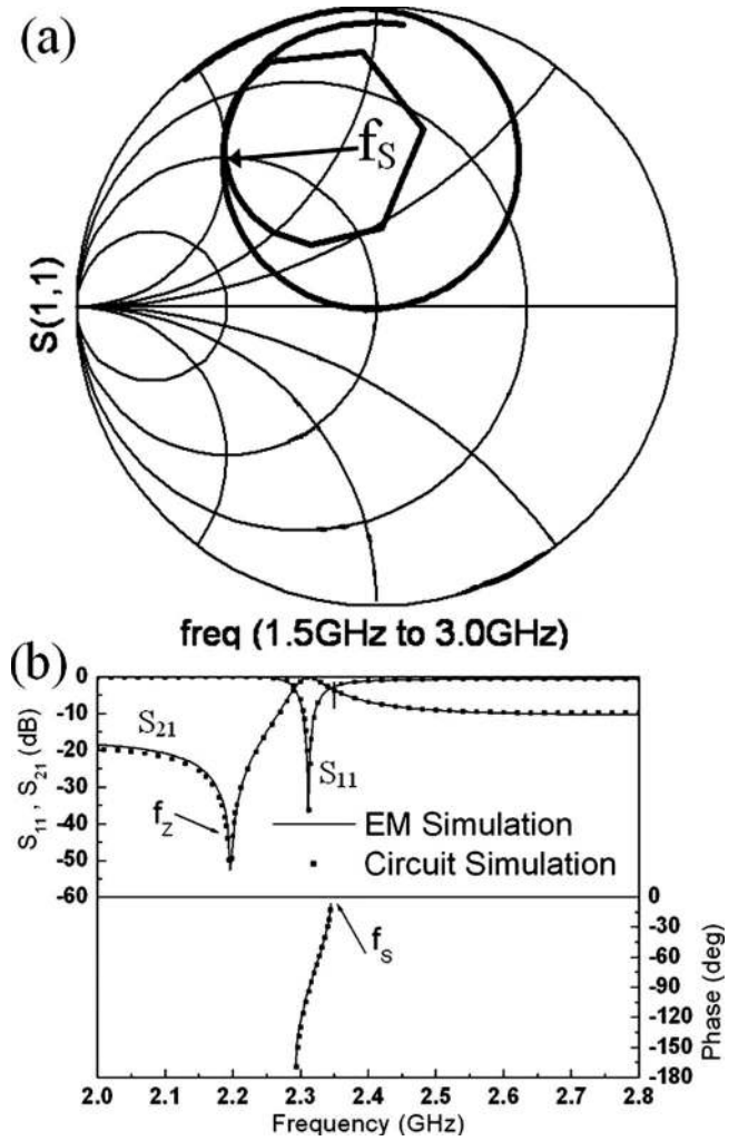
FIG. 4. Reflection coefficient on the Smith chart (a); frequency response (reflection, S_{11} , and transmission, S_{21} , coefficients) depicted in a decibel scale and the dispersion relation (b) for a left handed cell based on a microstrip structure. The considered substrate is Rogers RO3010 with thickness h = 1.27 mm and dielectric constant \epsilon_r = 10.2 . Relevant dimensions are ring width c = 0.6 mm; distance between the rings, d = 0.2 mm; and internal radius r = 2.4 mm. For the microstrip structure the strip line width is W_m = 7 mm and the length is D_m = 8.6 mm; the diameter of via is w_v = 0.4 mm. The results of the circuit simulation with extracted parameters are depicted using symbols.
