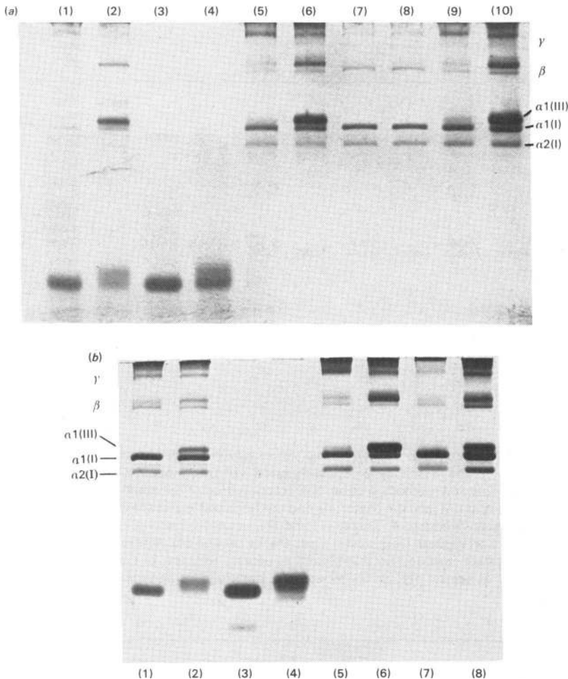
Fig. 1. SDS/polyacrylamide-gel-electrophoretic analysis of native collagens prepared from muscle epimysium and perimysium. Purified epimysium and perimysium from bovine muscle were digested with pepsin, and the native collagens released were fractionated by salt precipitation and analysed by SDS/polyacrylamide-gel electrophoresis as described in the Materials and methods section. (a) Epimysium peptic digest. Tracks (2), (4), (6), (8) and (10) were run in the presence of added 2-mercaptoethanol. Tracks (1) and (2), pepsin-insoluble material (21% of total); tracks (3) and (4), 7%-NaCl supernatant from 0.5M-acetic acid (residual pepsin); tracks (5) and (6), neutral-1 M-NaCl precipitate; tracks (7) and (8), neutral-1 M-NaCl supernatant; tracks (9) and (10), 2M-NaCl precipitate insoluble in 0.2M-NaCl at neutral pH. (b) Perimysium peptic digest. Tracks (1) and (2), pepsin-insoluble material (15% of total); tracks (3) and (4), 7%-NaCl supernatant from 0.5M-acetic acid (residual pepsin); tracks (5) and (6), 1 M-NaCl precipitate; tracks (7) and (8), 2M-NaCl precipitate insoluble in 0.2M-NaCl at neutral pH.
