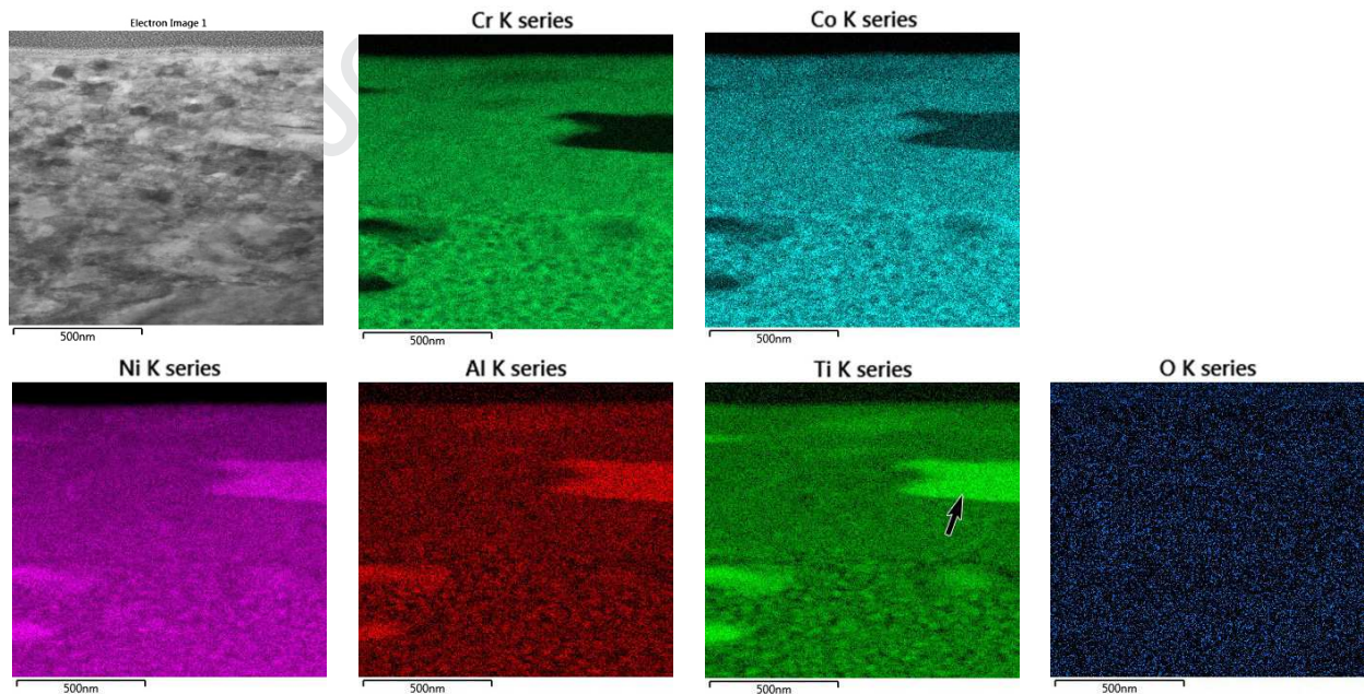
Figure 12 EDS maps from the top surface of the 'normal' region of the damaged specimen, showing a \sim 600 nm thick area without the original tertiary \gamma particles but with elongated secondary (arrowed) \gamma particle. In the region below that, the size of the small \gamma particles is \sim 30 nm, which is much smaller than the size of the original tertiary \gamma particles (71.5 nm) shown in fig. 2.
