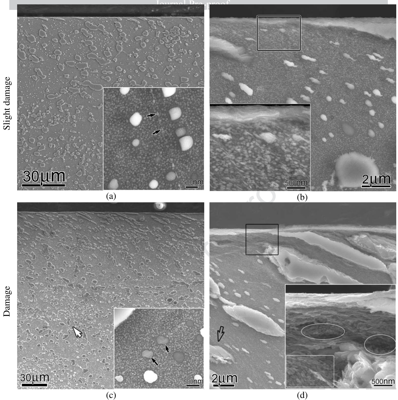
Figure 4 SEM images taken from the slightly damaged (a and b) and damaged (c and d) specimens. Inset to fig. 4a taken 33 \mu\text{m} away from the surface, showing a shear band (arrowed). Inset to fig. 4b taken from the marked area in no observable Fig. 4b, showing severely deformed secondary and tertiary \gamma precipitates and a \sim 400 nm wide layer (from the surface) with no observable \gamma precipitates. Inset to fig. 4c taken from the region arrowed in white (140 \mu\text{m} away from the surface), showing sheared secondary and tertiary \gamma precipitates. The arrow in fig. 4d indicates severely sheared \gamma precipitates; the wavelike bands observed in the inset to fig. 4d was taken from the marked rectangle in fig. 4d; the areas circled in white in the inset to fig. 4d show visible tertiary \gamma precipitates.
