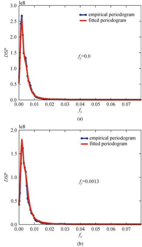
Fig. 22 Case #2: Cut of the periodograms in the X direction
