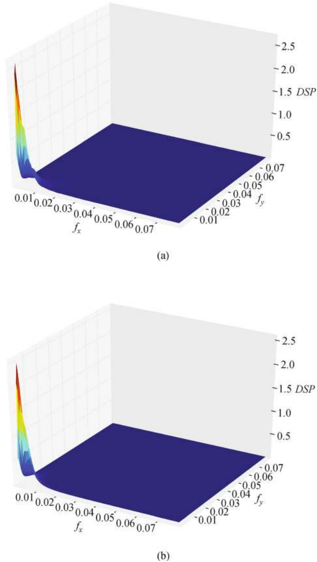
Fig. 21 Case #2: (a) Average empirical periodogram of the stress field at 3.5% macroscopic strain; (b) best fitted periodogram
