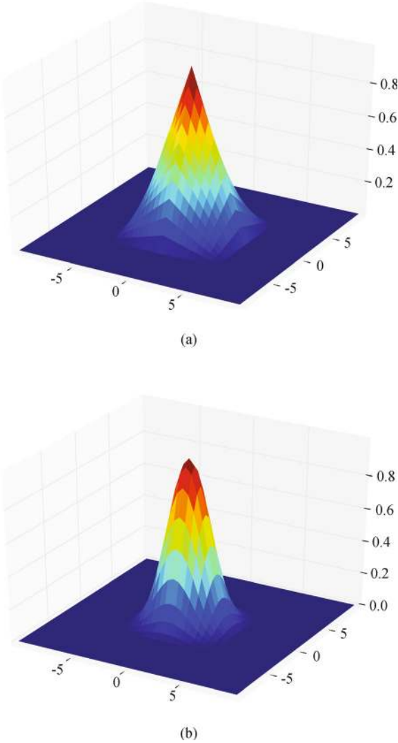
Fig. 2 (a) Bartlett window; (b) Blackman window
