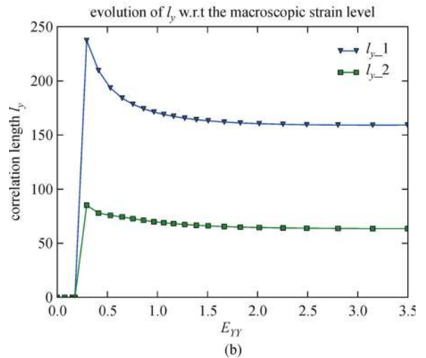
Fig. 18 Case #1: Evolution of the fitted correlation lengths in the X , Y directions with respect to the load level (macroscopic strain E_{YY} = 0, \dots, 3.5\% )
