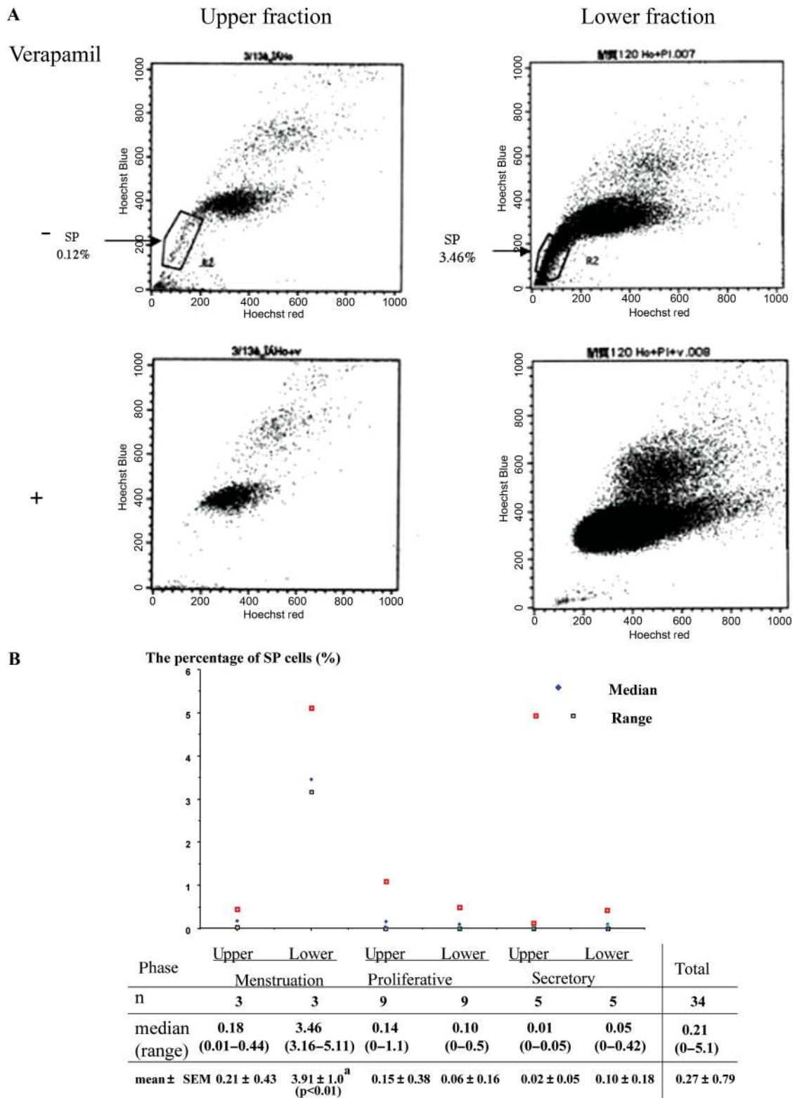
Figure 2. Side-population (SP) cells were present in the human endometrium. (A) Endometrial cells during menstruation (day 2) were stained with Hoechst 33342 and analysed by FACS. SP cells, which show a high level of dye efflux activity, were present in both the upper and lower fractions of the endometrium. Verapamil treatment increased the staining and made SP cells undetectable by FACS. (B) Summary of the SP cell percentage is shown. The graph shows the median and the range of scatter in each stage of the menstrual cycle. Data are also represented as the mean \pm SEM. (a) The SP cell percentage was significantly higher in endometrial cells in the lower fraction of the menstrual phase than in all other samples ( P < 0.01 ). (C) For analysis of the cell-surface markers of SP cells, cells stained with Hoechst 33342 dye were followed by incubation with FITC-conjugated anti-CD9 antibody and PE-conjugated anti-CD13 antibody. (a) Most SP cells were present in the CD9 - CD13 - fraction. (b) Cells in the CD9 - CD13 - fraction were enriched with SP cells. R1: viable cells gated by propidium iodide; R3: CD9 - CD13 - fraction. (D) (a) Morphologically, the SP cells were small and round in contrast to NSP cells. (b) Daughter cells were generated from a single SP cell (shown by arrows). (magnification: \times 500 ).
