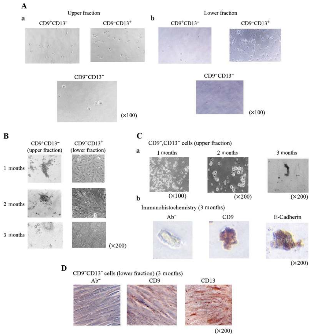
Figure 6. CD9^-CD13^- cells exhibited a similar phenotype to SP cells. (A) CD9^+CD13^- cells, CD9^-CD13^+ cells and CD9^-CD13^- cells were isolated by magnetic cell sorting from endometrial cells in the proliferative phase (day 7) digested with collagenase and were cultured on collagen-coated plates. (a) Cells from the upper fraction of the filter (cell density: CD9^+CD13^- cells, 2500\text{ cells cm}^{-2} , CD9^-CD13^+ cells, 2500\text{ cells cm}^{-2} , CD9^-CD13^- cells, 250\text{ cells cm}^{-2} ) (magnification: \times 100 ). (b) Cells from the lower fraction of the filter (cell density: CD9^+CD13^- cells, 500\text{ cells cm}^{-2} , CD9^-CD13^+ cells, 2500\text{ cells cm}^{-2} , CD9^-CD13^- cells, 250\text{ cells cm}^{-2} ) (magnification: \times 100 ) (B) Morphology of CD9^+CD13^- cells and CD9^-CD13^+ cells after 1, 2 and 3 months of culture. Both CD9^+CD13^- cells and CD9^-CD13^+ cells stopped proliferating after 2 months of culture (magnification: \times 100 ). (C). (a) Morphology of CD9^-CD13^- cells from the upper fraction after 1, 2, and 3 months of culture (magnification: 1 months \times 100 , 2, 3 months \times 200 ). (b) The expression of CD9 and E-cadherin in cells generated from CD9^-CD13^- cells from the upper fraction after 3 months of culture was investigated by immunohistochemistry (magnification: \times 200 ). (D) Morphology and expression of CD9 and CD13 by immunohistochemistry was shown in CD9^-CD13^- cells from the lower fraction after 3 months of culture (magnification: \times 200 ). Ab - represents no added antibody.
