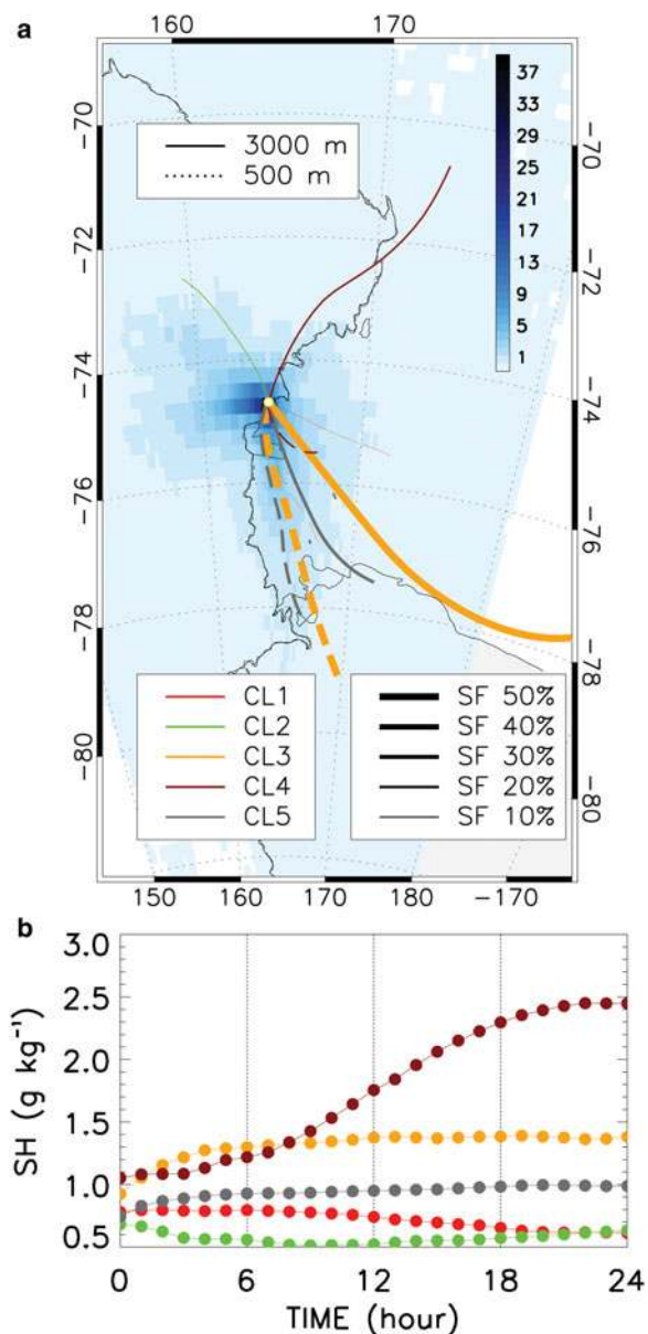
Fig. 6. The main pattern of 1 d back-trajectories ending at 3000 m over Mario Zucchelli Station. (a) The number of back-trajectories transited over each lon-lat box of 0.5^\circ \times 0.25^\circ , during the whole period (computed hourly from 6 November to 31 January, during 2015–16, 2016–17, 2017–18 and 2018–19 summer campaigns) is reported in a blue color scale. The map is expressed in percent with respect to the number of total back-trajectories considered. Overlying, the mean trajectories, representative of each cluster obtained in the analysis, are reported in different colors. Cluster analysis is applied only to trajectories at 3000 m (solid lines) and 500 m (dashed lines) associated with snowfall events at the site ( \text{SF} > 0 ). The width of the trajectories line represents the percentage of the snowfall related to each cluster. (b) The mean specific humidity ( \text{g kg}^{-1} ) along the trajectory is reported, for each cluster.
