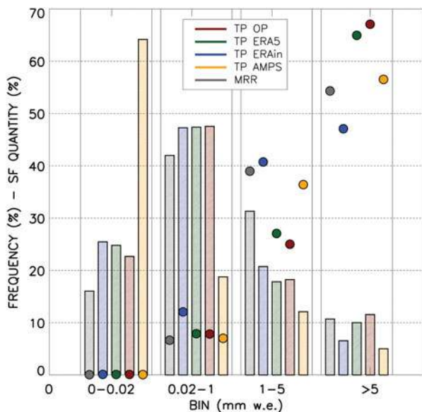
Fig. 9. Comparison between observations and models. Frequency (%), dashed bars) and quantities (%), filled points) of model total precipitation (TP) cumulated on a daily basis, grouped for events from 0 to 0.02, 0.02–1, 1–5, >5 mm w.e.; gray, red, green, blue and orange are referred to MRR, Operational (OP), ERA5, ERA Interim (ERAIn) and AMPS, respectively.
