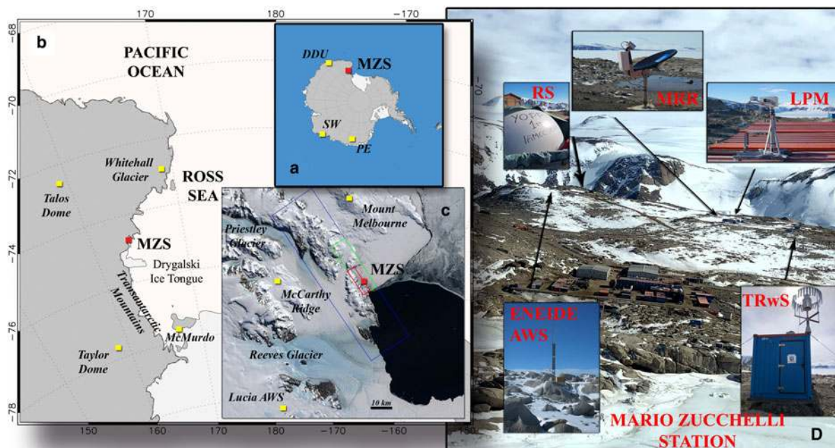
Fig. 1. Map of the studied area. (a) Map of Antarctica with the position of Mario Zucchelli (MZS), Princess Elisabeth (PE), Dumont d'Urville (DDU) and Syowa (SW) stations. (b) Location and coastal profile of the area of Victoria Land (Antarctica). (c) A clear sky Aqua MODIS image (250 m resolution) of the Terra Nova Bay (TNB) area in Victoria Land. Red and yellow points indicate the positions of Mario Zucchelli Station (MZS), automatic weather station (AWS) Lucia (Larsen Glacier), McCarthy Ridge ice core site and Mount Melbourne, respectively. Colored rectangles show model nearest mesh of ECMWF ERA Interim, ERA5 and Operational products (green, blue and red, respectively) including MZS (red square). (d) Photo of MZS with positions and images of the instruments (AWS Eneide, MRR Metek radar, LPM OASI Thies Clima optical disdrometer and TRwS MPS weighing snow gauge, and radiosounding launcher) used for this study.
