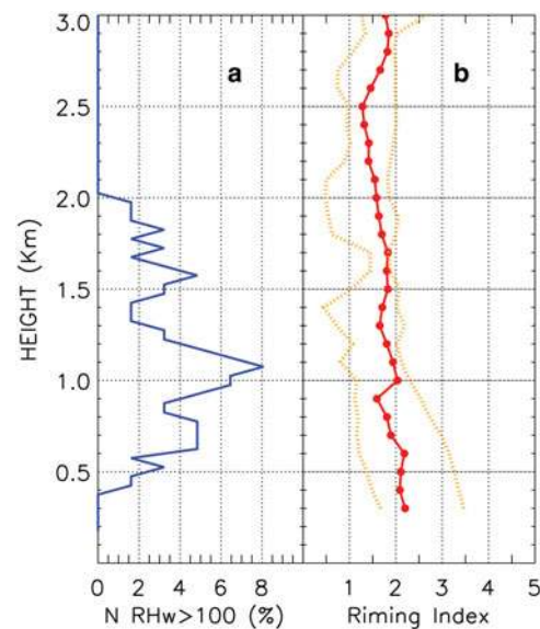
Fig. 7. (a) Number of events (%) for relative humidity with respect to water (RHw) \geq 100\% for each profile height levels as measured by radiosounding launched during precipitation events. (b) Median, 10 and 90 percentile values profile (red thick and orange dotted lines, respectively) of riming index calculated as Mosimann (1995) using mean fall velocity ( W ) sampled by MRR radar during the co-located radiosounding launches used in (a). Scale values on x-axis represent the degree of riming (1 = lightly rimed, 2 = moderately rimed, 3 = densely rimed, 4 = heavily rimed and 5 = graupel).
