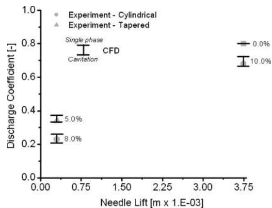
FIG. 4. Measured and predicted nozzle discharge coefficient as function of needle lift.
