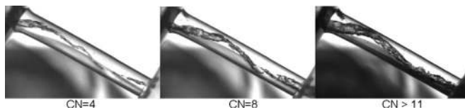
FIG. 10. Effect of CN of string cavitation structure inside the tapered injection hole (needle lift: 0.3 \times 10^{-3} m and Re=38\,000 ).
