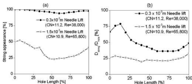
FIG. 15. Effect of the needle lift on (a) string appearance along the hole length expressed as percentage of time and (b) normalized mean string diameter along the hole length.
