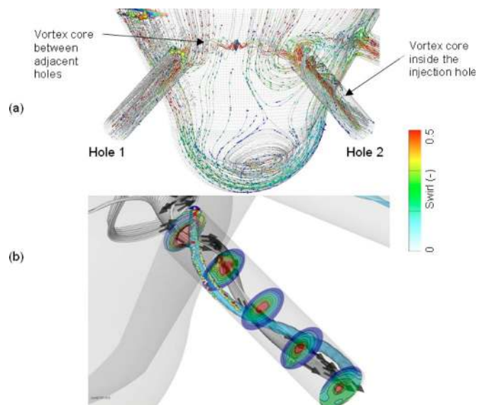
FIG. 9. (Color online) Model predictions for the original VCO nozzle using slightly eccentric needle position. Calculations indicate (a) formation of a strong vortex formed in between adjacent holes and (b) the vortex core inside the injection hole can be linked with the area where string cavitation has been observed.
