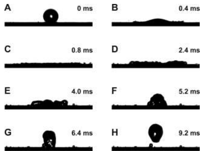
Figure 9. Impact and rebound of a 1.59 mm drop of water onto a cold (-10°C) superhydrophobic layer with 3.3 m/s impact velocity. The drop partially breaks up [121].
