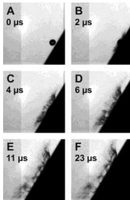
Figure 10. Splash of a drop of 194 μm diameter on a superhydrophobic surface at an impact velocity 34 m/s [121].
