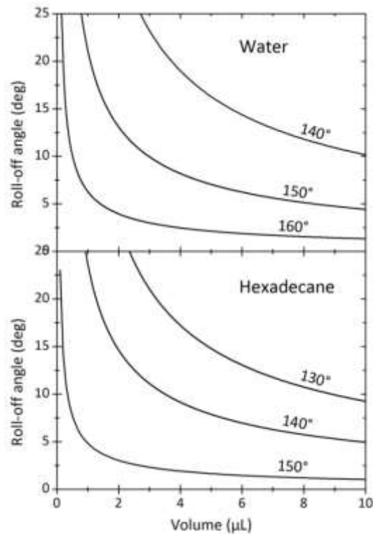
Figure 6. Maximal roll-off angles possible for a drop of water ( \rho=997 \text{ kg/m}^3 , \gamma=0.0720 \text{ N/m} ) and hexadecane ( \rho=770 \text{ kg/m}^3 , \gamma=0.0271 \text{ N/m} ) at 25^\circ\text{C} at a given receding apparent contact angle of 130^\circ , 140^\circ , 150^\circ , and 160^\circ versus the drop volume. A spherical drop shape was assumed and Eqs. (3-4) with \Delta\Theta \approx 0.55(180^\circ - \Theta_r^{app}) were applied. Above the plotted lines the drop certainly rolls off the layer.
