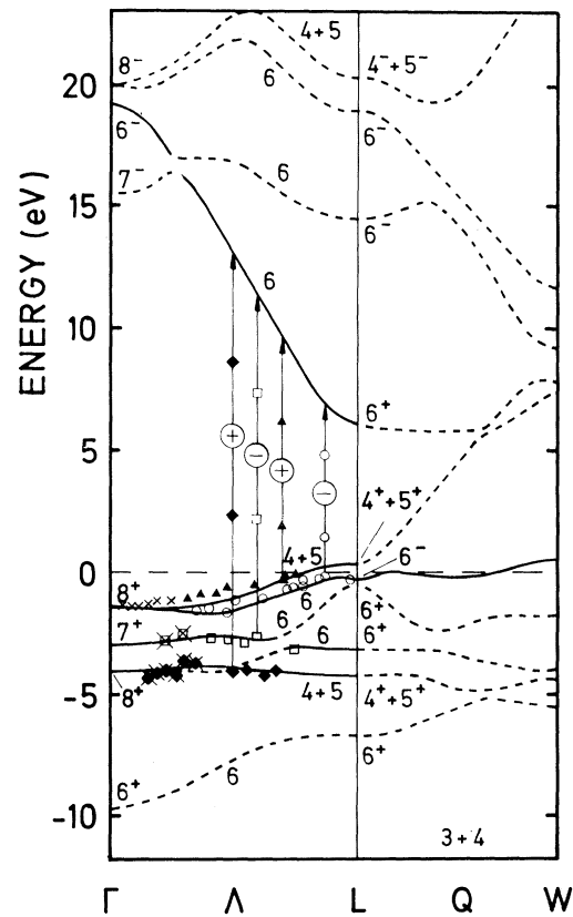
FIG. 2. Symmetry-resolved band mapping of Pt (Ref. 11) in comparison with the calculated band structure: the band mapping procedure used the calculated final band No. 7 for photon energies < 20 eV and a free-electron parabola (not shown) with V_0 = -1.85 eV and m^* = 1.10m_e for h\nu > 20 eV, which yields the mapping points without and with crosses, respectively. The mapping points (filled for positive polarization and open for negative) have been obtained by a combination of the intensity and spin-polarization results, partly shown in Fig. 3.
