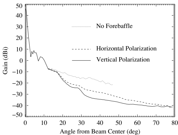
Figure 17. Azimuthally averaged sidelobe response for the 100 GHz central feed. A forebaffle with an absorptive lining cuts in at 15.5^\circ and provides up to an additional \sim 15 dB attenuation. When the telescope is at its lowest elevation of 50^\circ , the lip of the outer ground screen is \sim 30^\circ from the beam center of the central feed.
