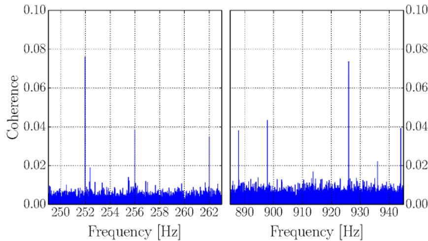
Figure 10: The coherence between the L1 GW readout signal and data from a magnetometer in the central building at LLO over one week of March 2010. 2 Hz and 16 Hz harmonics were seen to be coherent at numerous locations across the operating band of both interferometers, affecting the sensitivity of long-duration GW searches.
