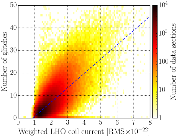
Figure 7: Correlation between low SNR glitches in the GW data, and current in the test mass coil at H1. This correlation is indicative of the Barkhausen effect.
