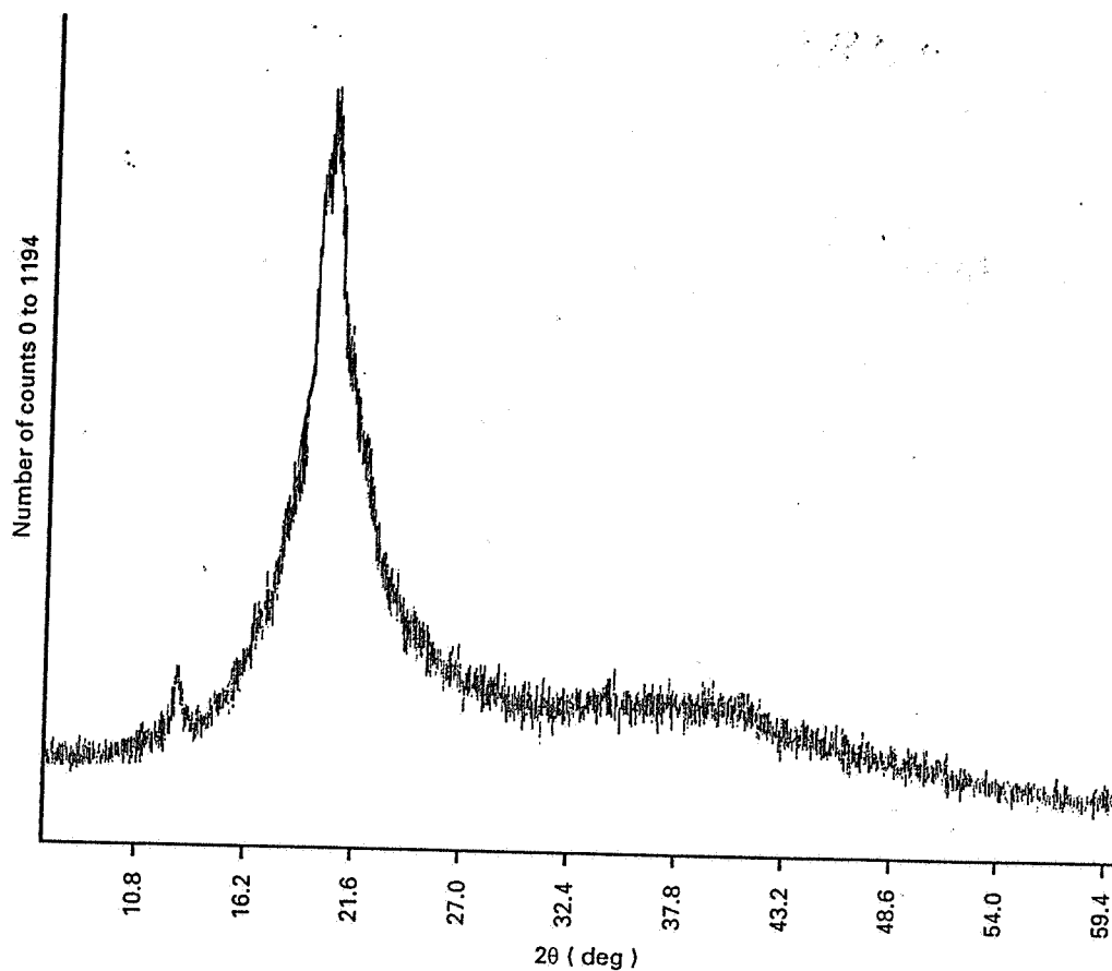
Figure 3 XRD pattern for SEVA-C. Peaks detected do not match any standard JCPDS file. Based on these patterns a crystallinity value of 45–50% was estimated for SEVA grades.
