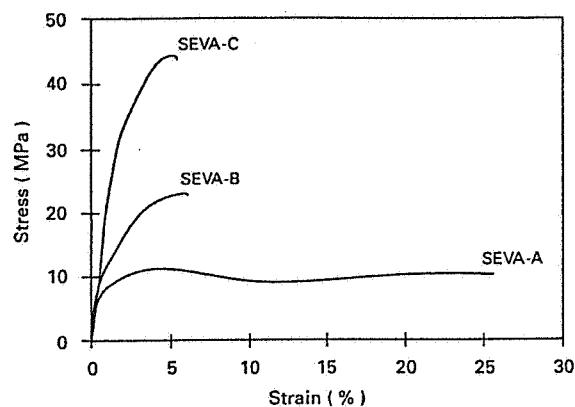
Figure 2 Stress versus strain plot for SEVA polymers as obtained in the tensile tests.
