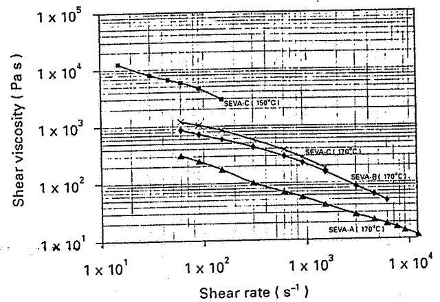
Figure 6 Flow curves for SEVA polymers.
