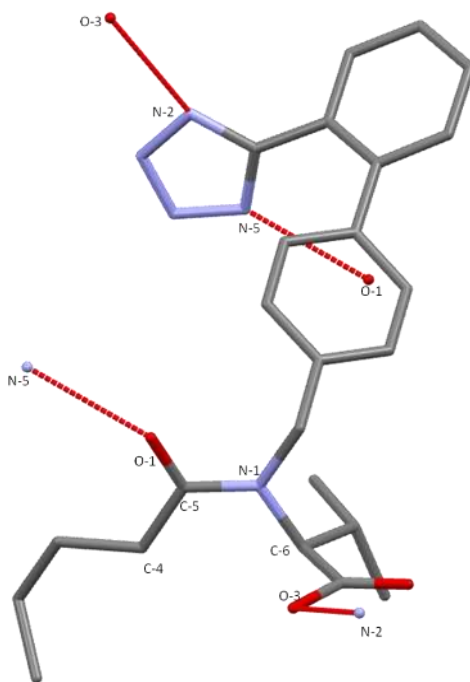
Figure 1. (A) Chemical structure of valsartan ( N -[ p -( o -1 H -tetrazol-5-yl)phenyl]benzyl]- N -valeryl- L -valine) with all carbons and nitrogens numbered. Numbering scheme used as in Refs. 20, 21 The dihedral angle C-6-N-1-C-5-O-1, \tau , that determines the amide cis ( \tau \approx 180^\circ ) vs trans ( \tau \approx 0^\circ ) conformation, as defined in Ref. 21 , is shown. (B) The structure of the independent molecule of valsartan in the asymmetric unit and hydrogen bonding adapted from Ref. 20 The \tau torsion angle is \sim 171^\circ , corresponding to the cis isomer. Hydrogens are omitted for clarity.
