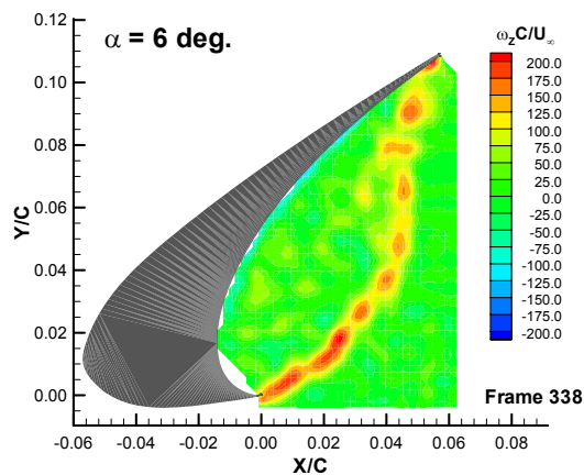
Figure 15b: Instantaneous spanwise vorticity (Cove State 2).
