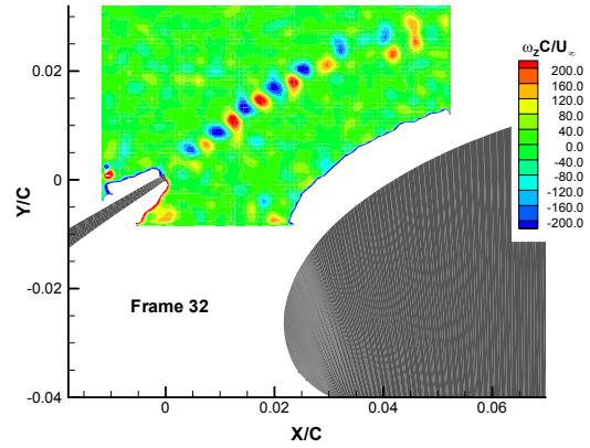
Figure 23b: Instantaneous spanwise vorticity (Slat State 1).
