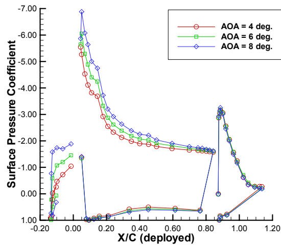
Figure 4: Surface pressure distributions along model centerline.
