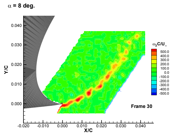
Figure 22: Instantaneous spanwise vorticity.
