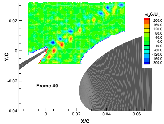
Figure 25b: Instantaneous spanwise vorticity (Slat State 3).
