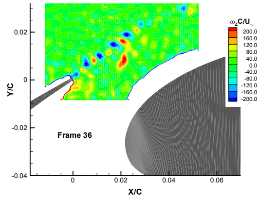
Figure 24b: Instantaneous spanwise vorticity (Slat State 2).
